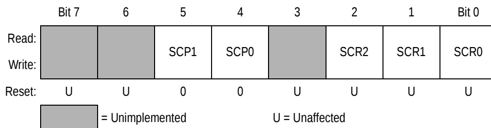
Figure 10-9. Baud Rate Register (Baud)
