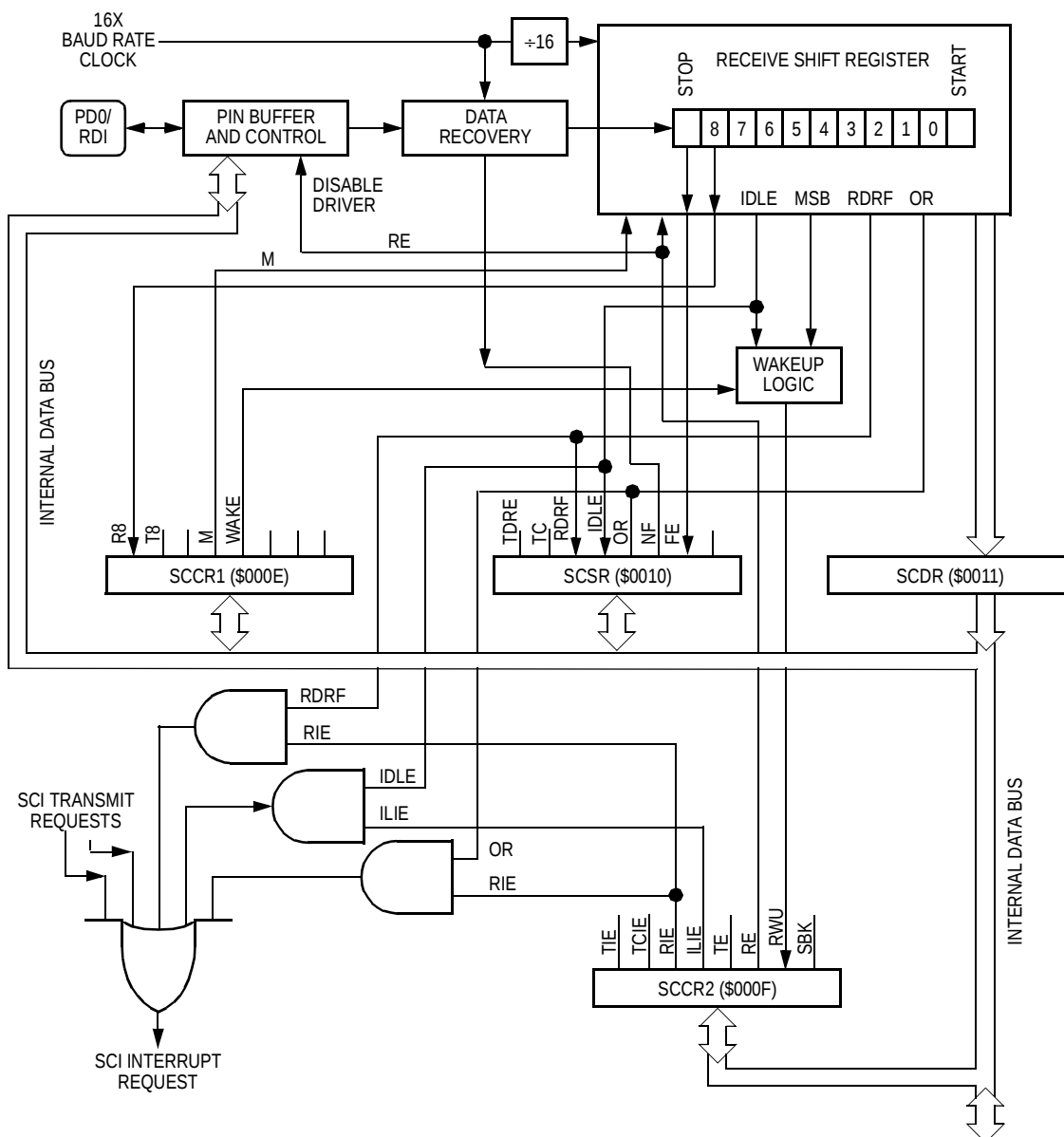
Figure 10-4. SCI Receiver
