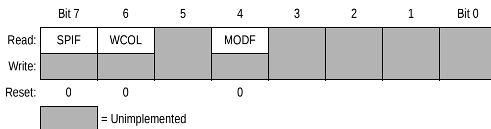
Figure 11-9. SPI Status Register (SPSR)
