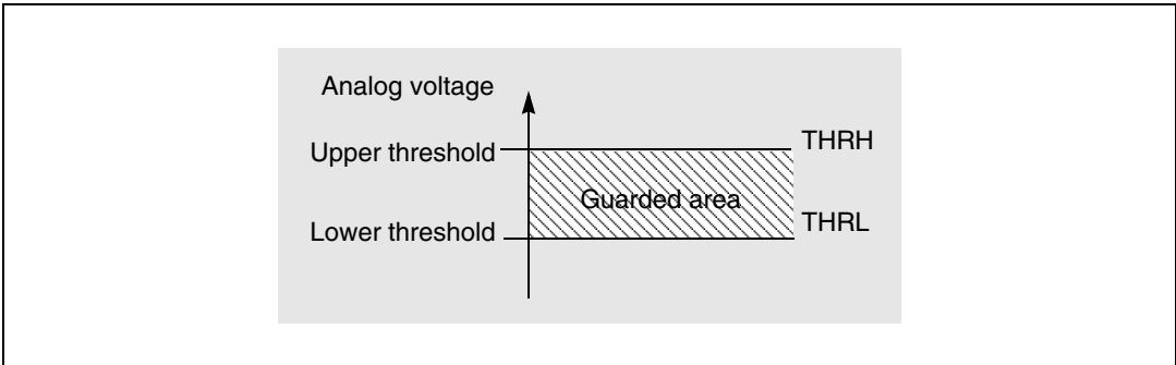
Figure 23-6. Guarded area
