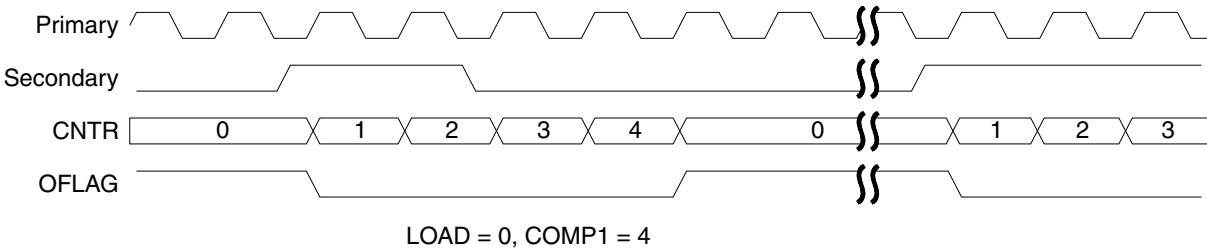
Figure 26-26. One-Shot mode (length = 1)
