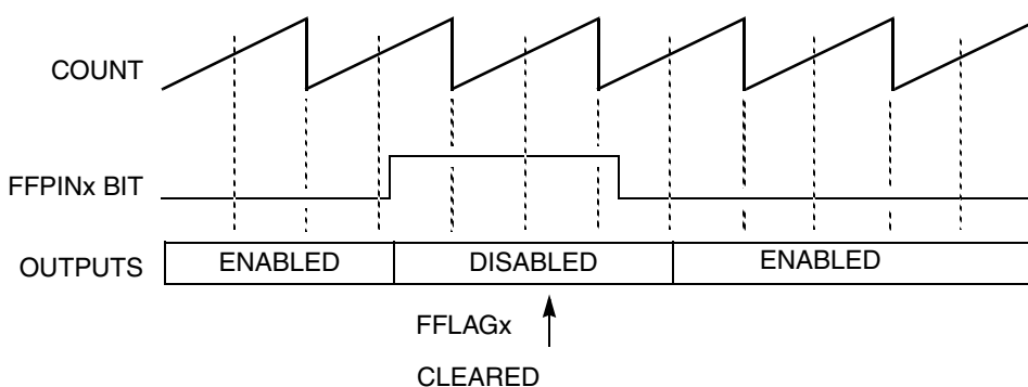
Figure 25-53. Manual fault clearing (FSAFE = 1)
