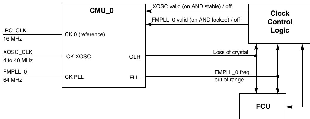
Figure 4-11. MPC5602PCMU
