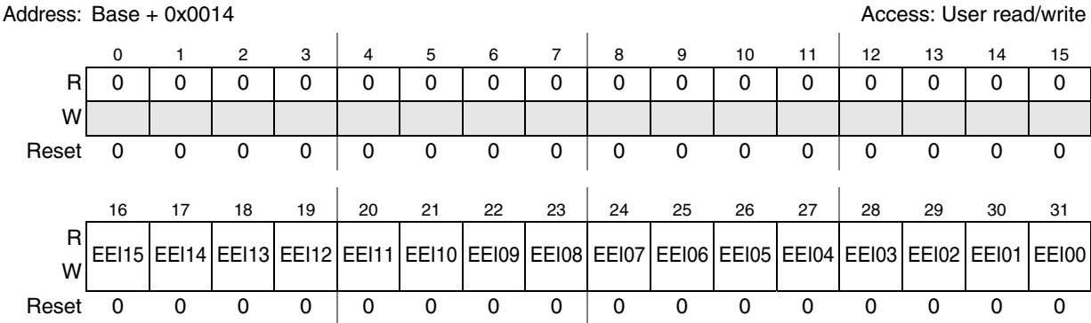
Figure 18-5. eDMA Enable Error Interrupt Low Register (EDMA_EEIRL)
