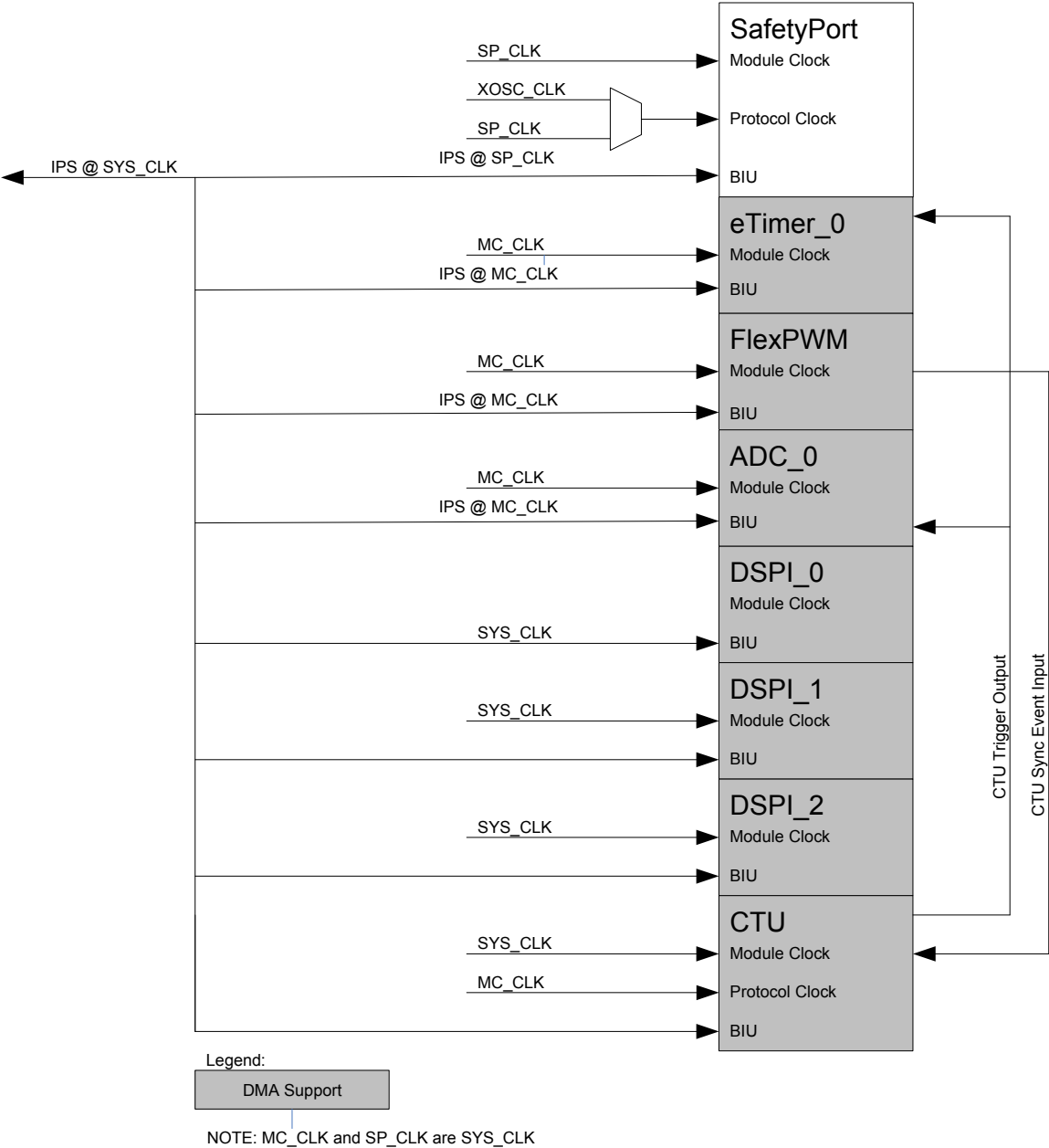
Figure 4-2. MPC5602P system clock distribution Part A
