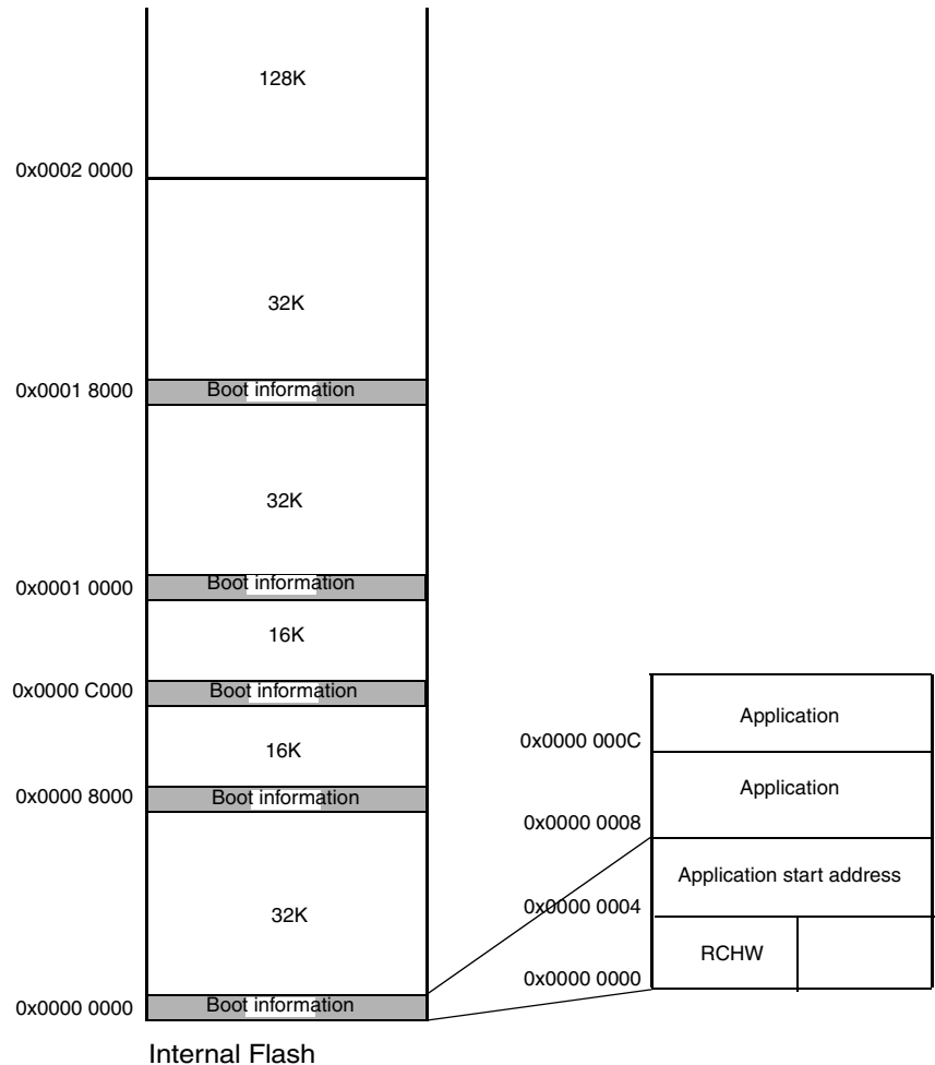
Figure 33-3. MPC5602P Flash partitioning and RCHW search
