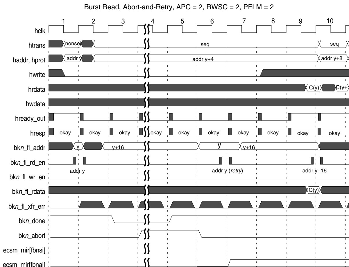
Figure 17-7. 3-cycle access, terminate-and-retry with BK_n\_RWWC = 10x
