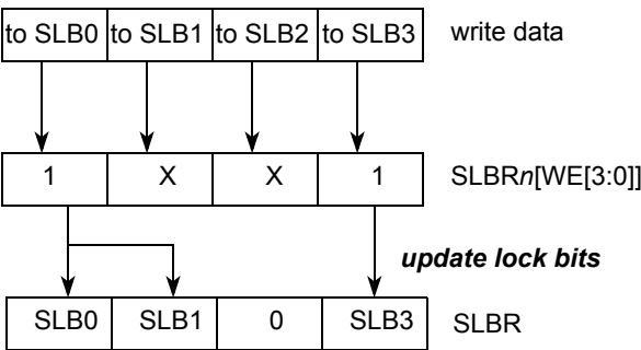
Figure 27-8. Change lock settings for mixed protection
