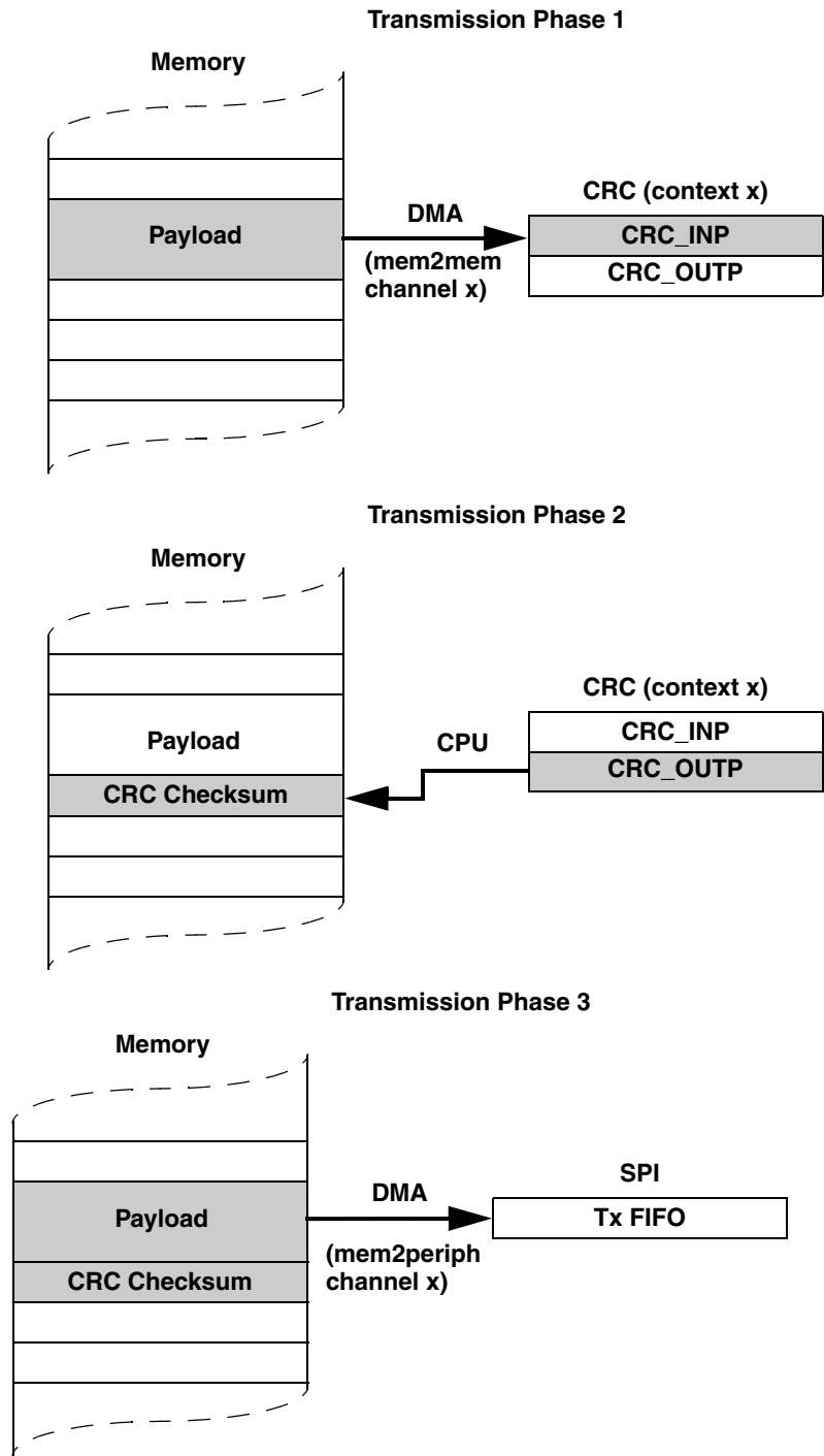
Figure 32-8. DMA-CRC Transmission Sequence
