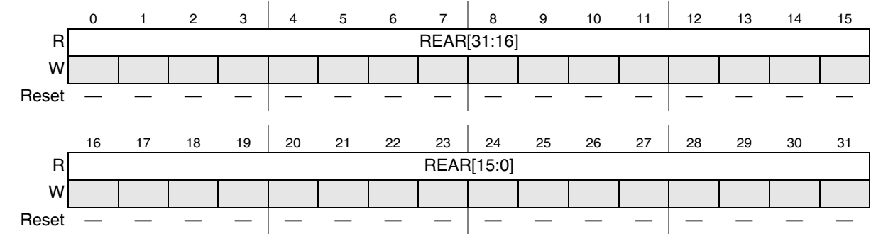
Figure 15-16. RAM ECC Address register (REAR)
