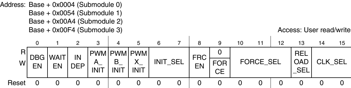
Figure 25-5. Control 2 Register (CTRL2)
