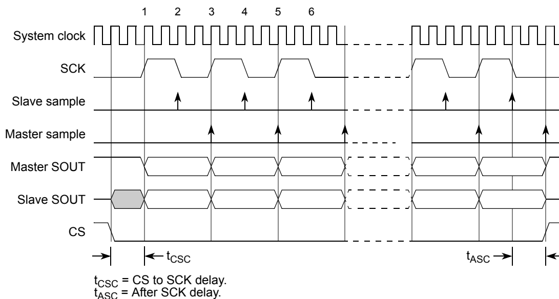
Figure 20-19. DSPI modified transfer format (MTFE = 1, CPHA = 1, f_{SCK} = f_{sys} / 4 )
