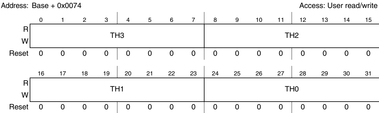
Figure 24-22. FIFO threshold register (FTH)
