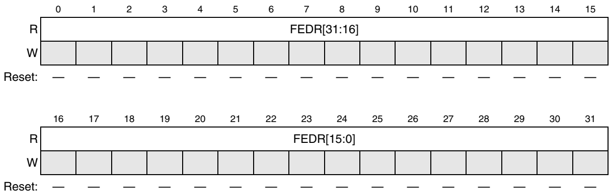
Figure 15-15. Flash ECC Data register (FEDR)
