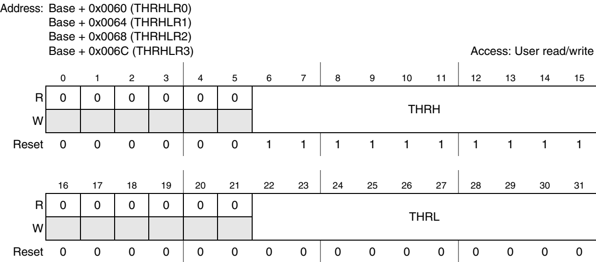
Figure 23-17. Threshold Register (THRHLR[0:3])
