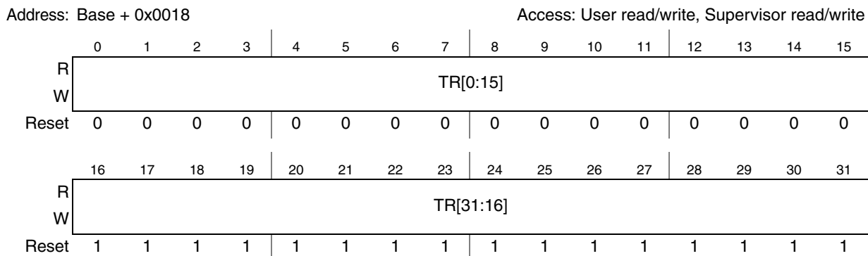
Figure 28-9. Timeout Register (FCU_TR)
