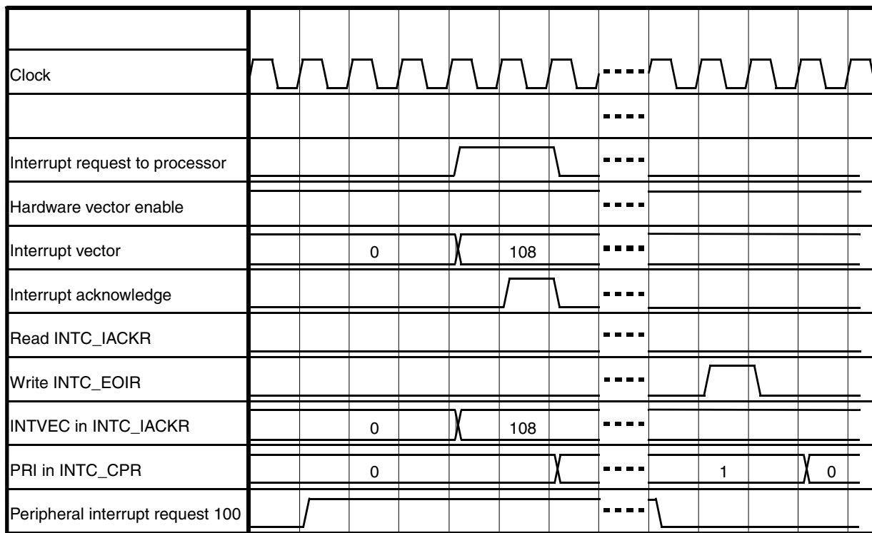
Figure 9-11. Hardware vector mode handshaking timing diagram
