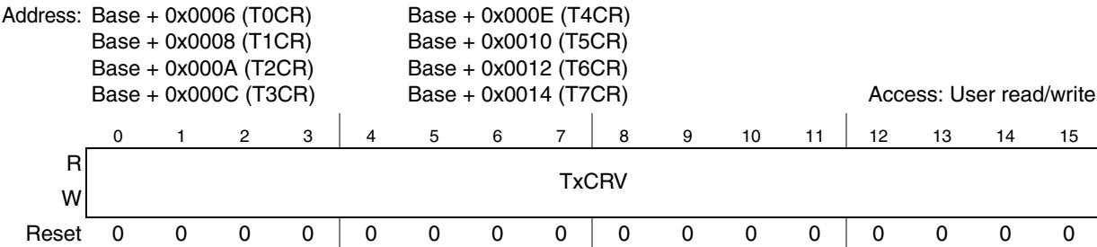
Figure 24-11. Trigger x Compare Register (TxCR, x = 0...7)
