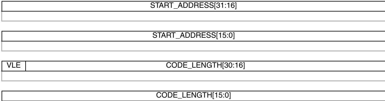
Figure 33-6. Start address, VLE bit and download size in bytes
