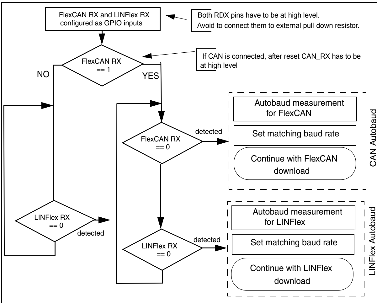
Figure 33-9. BAM Autoscan code flow
