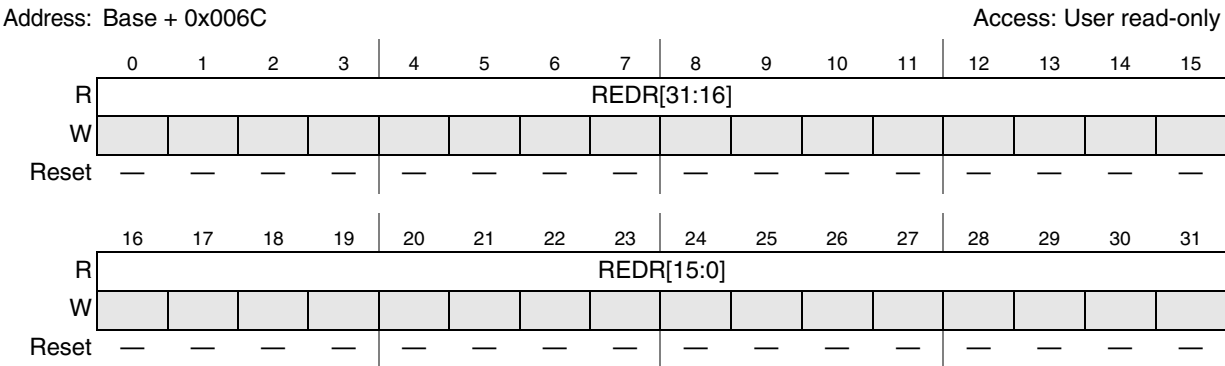
Figure 15-20. Platform RAM ECC Data register (PREDR)
