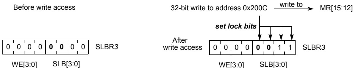
Figure 27-10. Enable locking for protected and unprotected addresses
