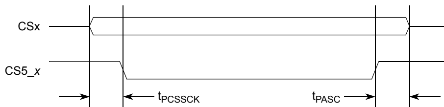
Figure 20-15. Peripheral Chip Select strobe timing
