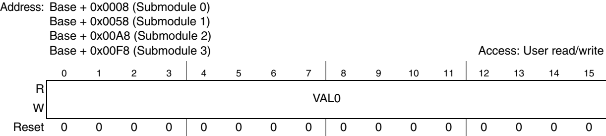
Figure 25-7. Value Register 0 (VAL0)
