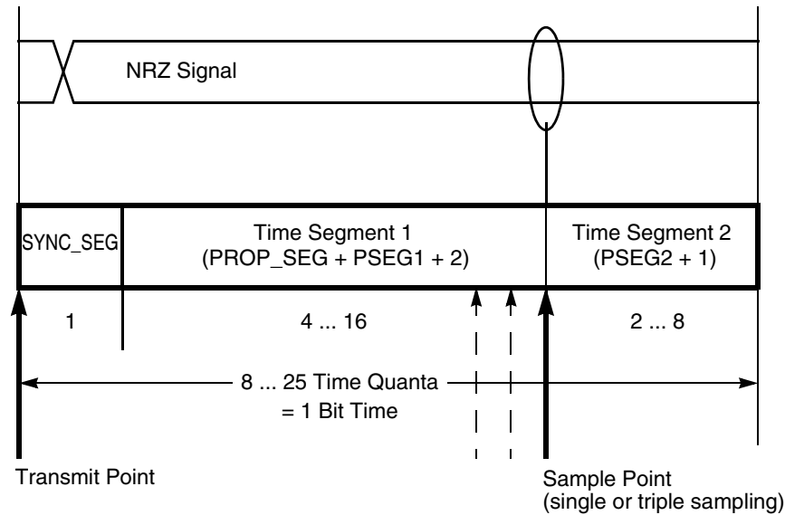
Figure 22-16. Segments within the bit time
