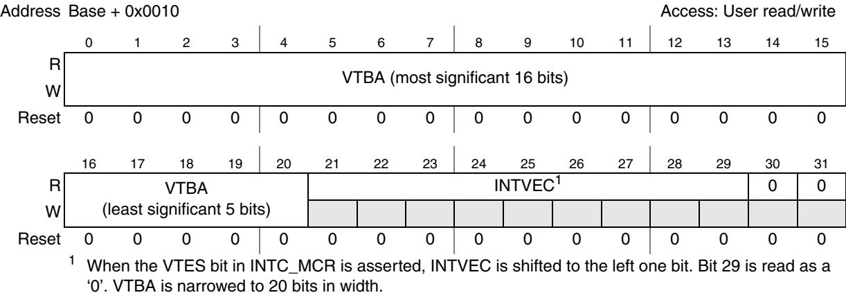
Figure 9-4. INTC Interrupt Acknowledge Register (INTC_IACKR)
