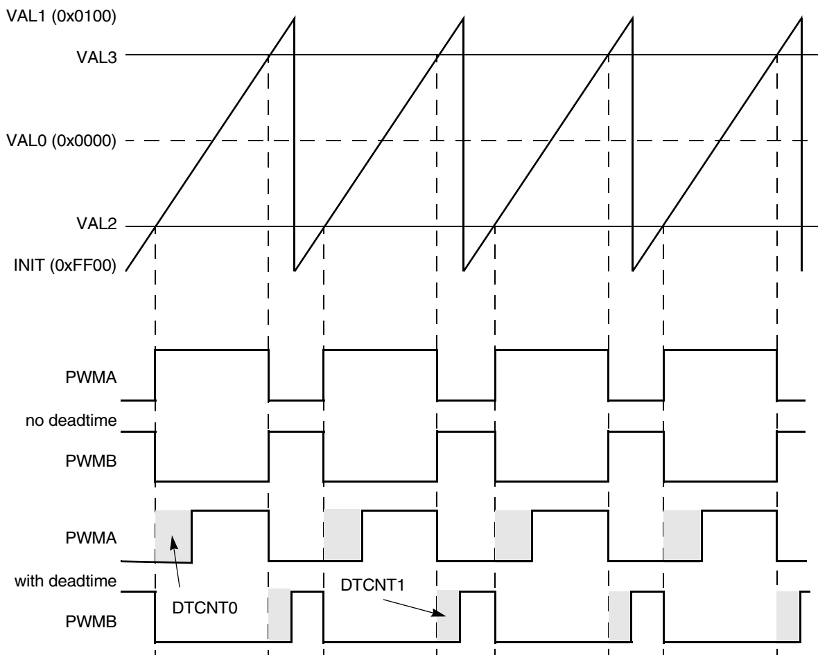
Figure 25-45. Deadtime insertion
