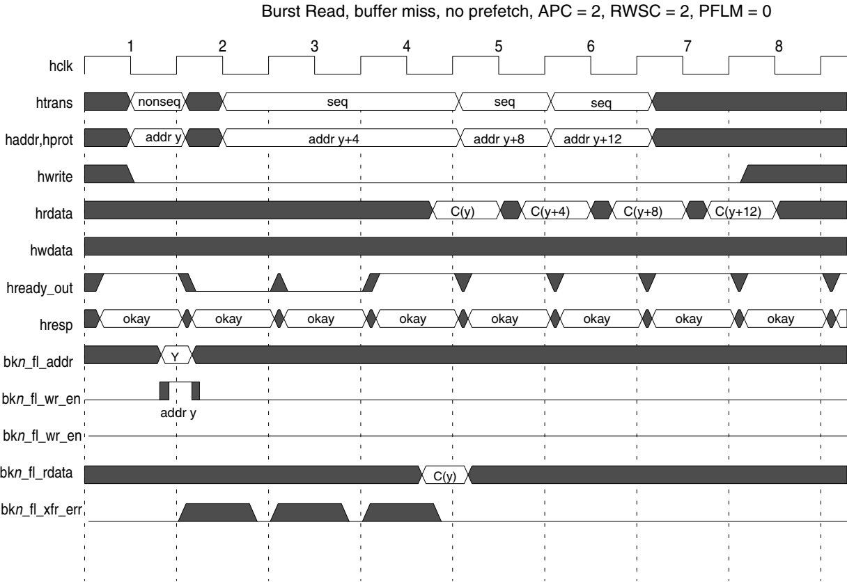
Figure 17-4. 3-cycle access, no prefetch, buffering enabled
