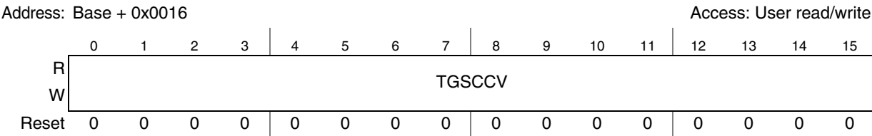
Figure 24-12. TGS Counter Compare Register (TGSCCR)
