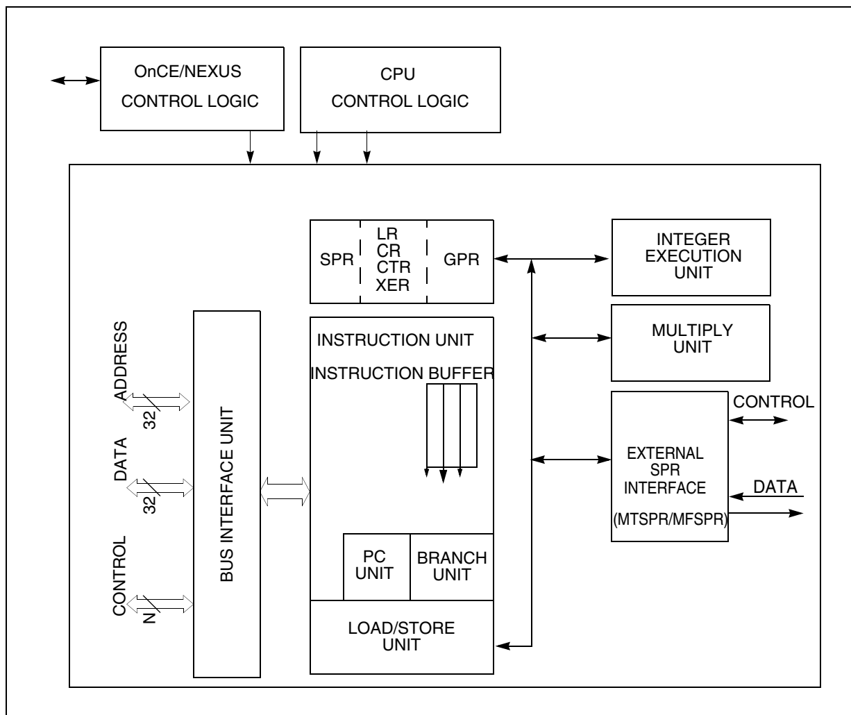
Figure 12-1. e200z0 block diagram
