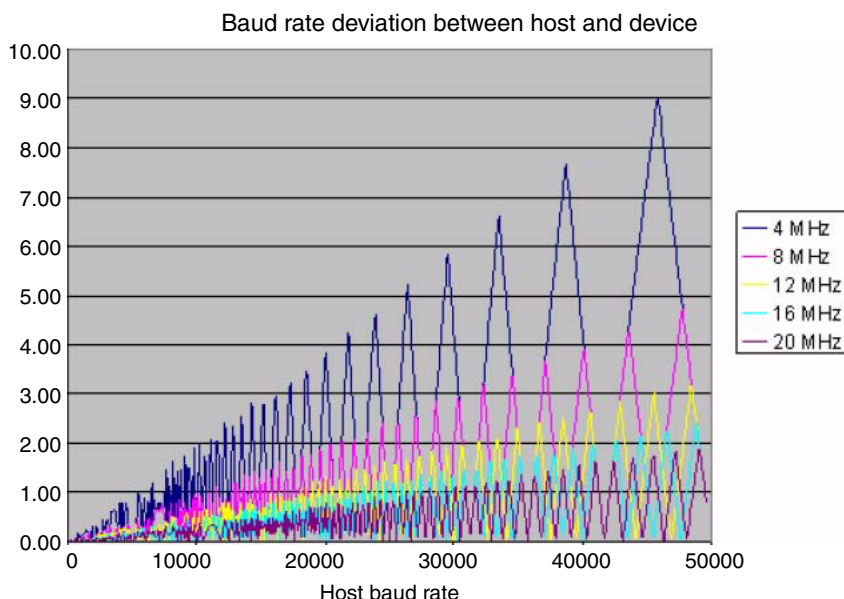
Figure 33-12. Baud rate deviation between host and MPC5602P
