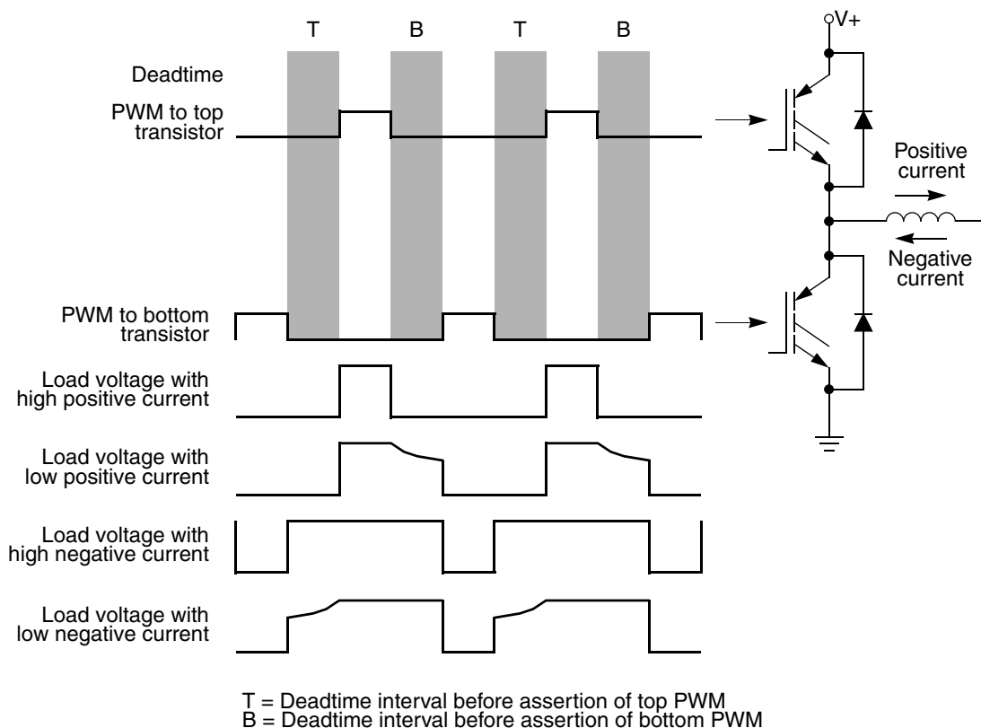
Figure 25-48. Output voltage waveforms
