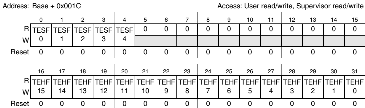
Figure 28-10. Timeout Enable Register (FCU_TER)
