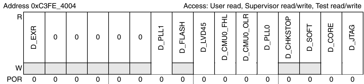
Figure 8-4. Functional Event Reset Disable Register (RGM_FERD)
