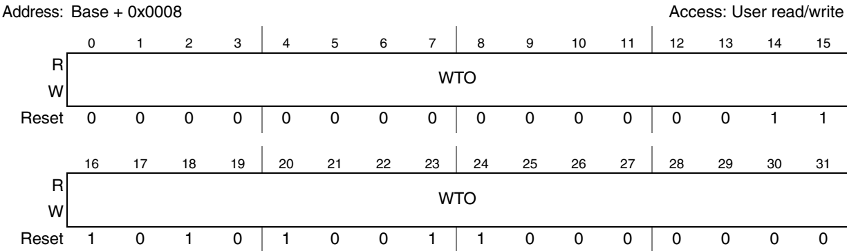
Figure 27-13. SWT Time-Out register (SWT_TO)
