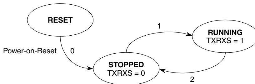
Figure 20-13. DSPI start and stop state diagram
