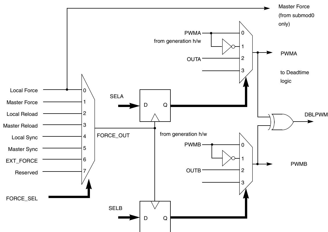
Figure 25-41. Force out logic
