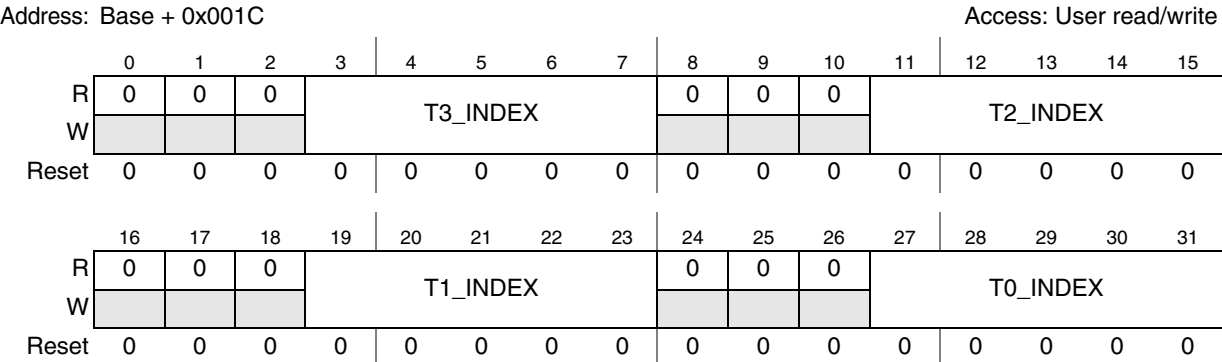
Figure 24-14. Commands list control register 1 (CLCR1)
