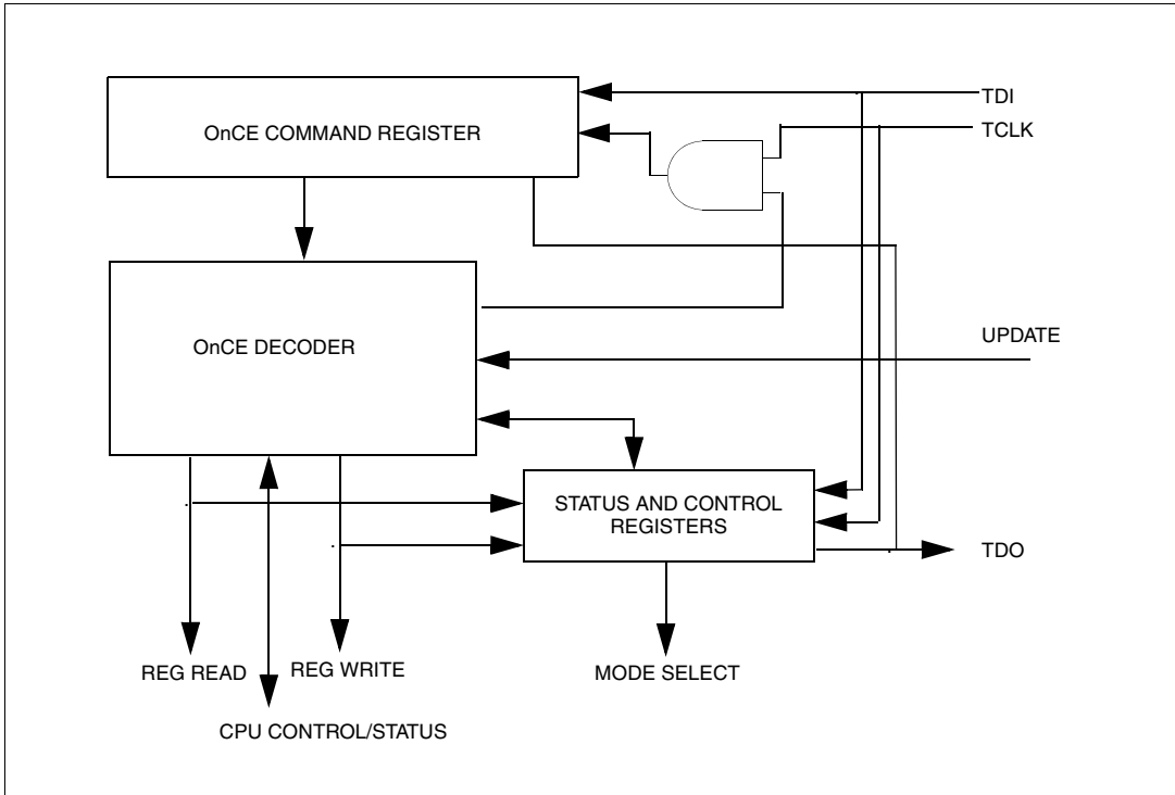
Figure 36-12. e200z0h OnCE Controller and Serial Interface
