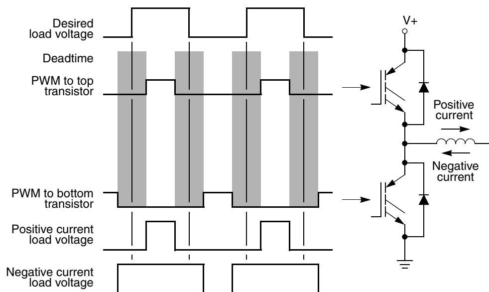
Figure 25-46. Deadtime distortion
