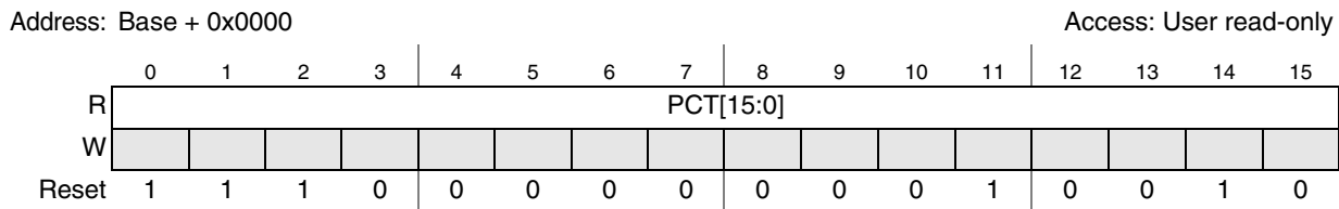
Figure 15-1. Processor core type (PCT) register
