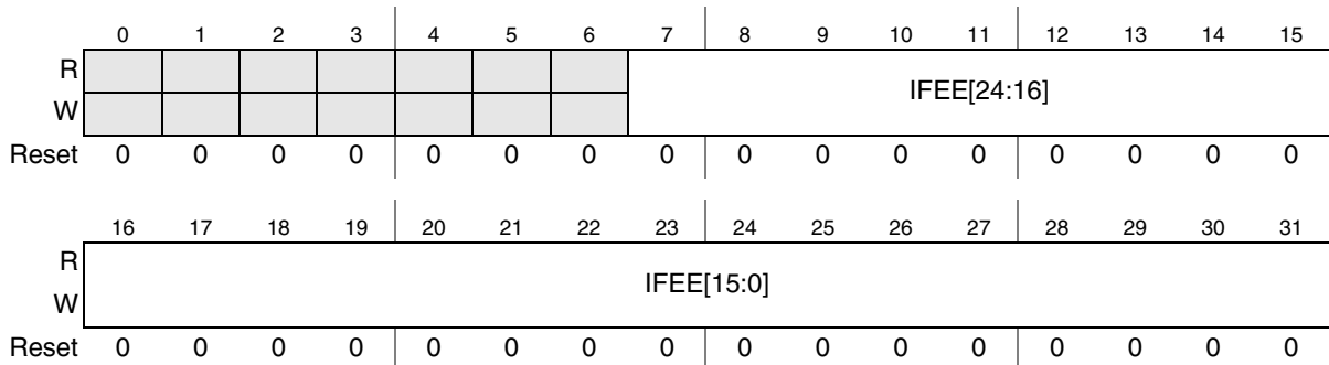
Figure 11-8. Interrupt Falling-Edge Event Enable Register (IFEER)
