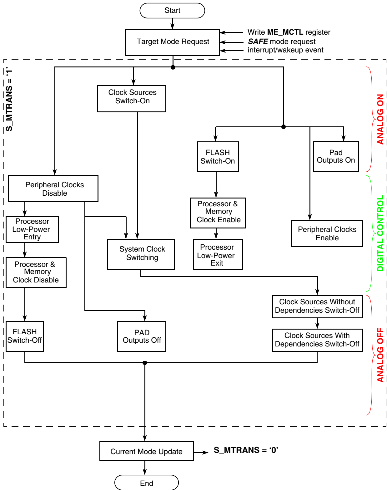
Figure 7-23. MC_ME Transition Diagram
