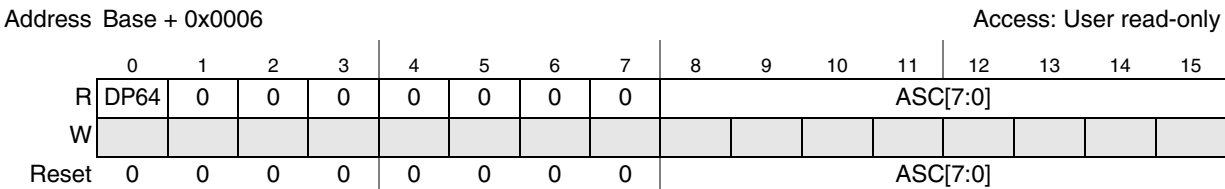
Figure 15-4. Platform XBAR Slave Configuration (PLASC) register
