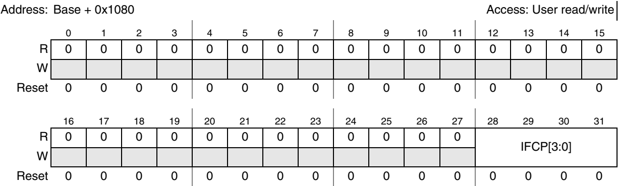
Figure 11-18. Interrupt Filter Clock Prescaler Register (IFCPR)
