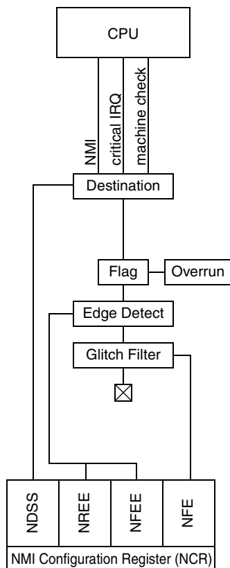
Figure 29-3. NMI pad diagram
