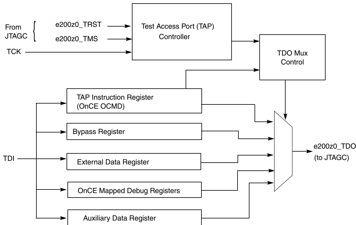
Figure 35-6. e200z0 OnCE block diagram
