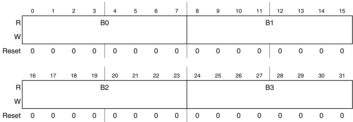
Figure 36-3. DVC1, DVC2 Registers
