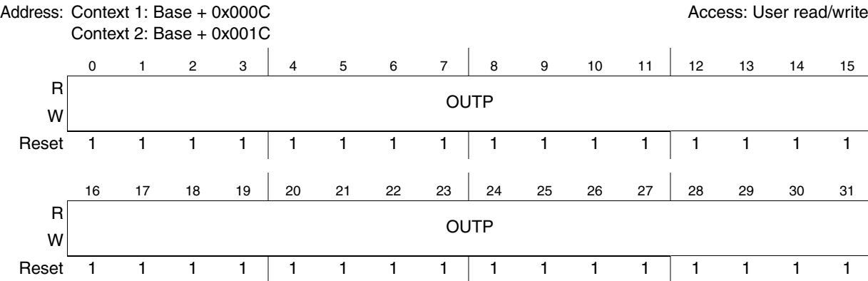
Figure 32-7. CRC Output Register (CRC_OUTP)
