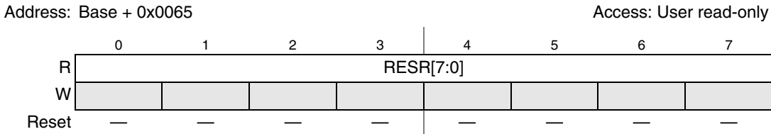
Figure 15-17. RAM ECC Syndrome Register (RESR)
