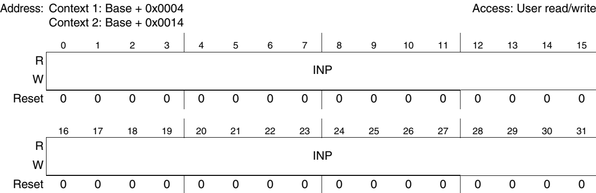
Figure 32-5. CRC Input Register (CRC_INP)
