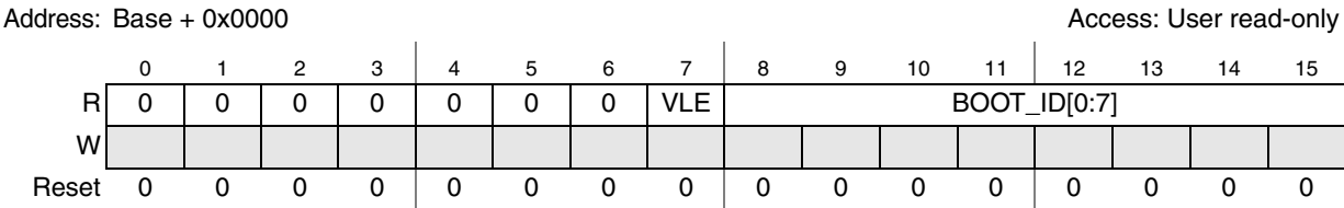
Figure 33-2. Reset Configuration Half Word (RCHW)
