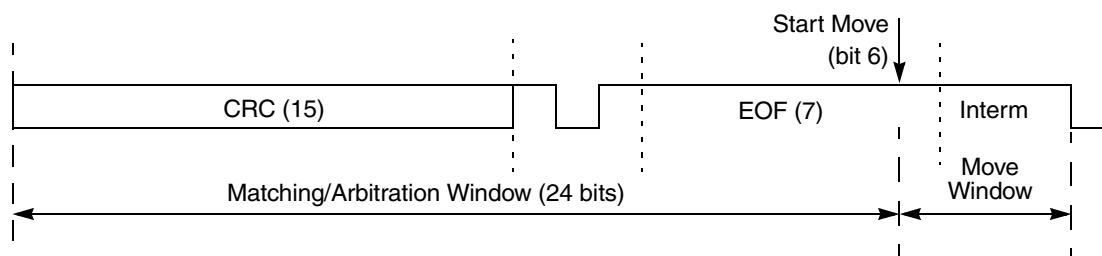
Figure 22-17. Arbitration, match, and move time windows
