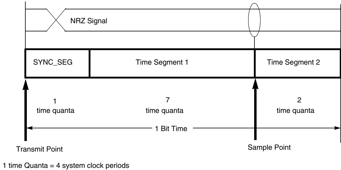
Figure 33-8. FlexCAN bit timing
