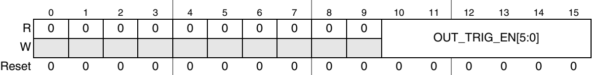
Figure 25-17. Output Trigger Control register (TCTRL)
