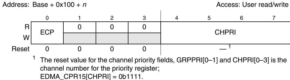
Figure 18-17. eDMA Channel n Priority Register (EDMA_CPR n )
