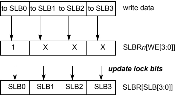
Figure 27-7. Change lock settings for 32-bit protected addresses
