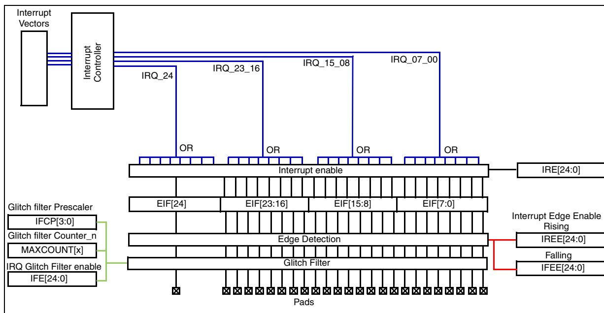
Figure 11-20. External interrupt pad diagram
