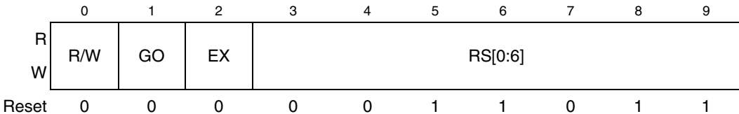
Figure 35-7. OnCE Command register (OCMD)
