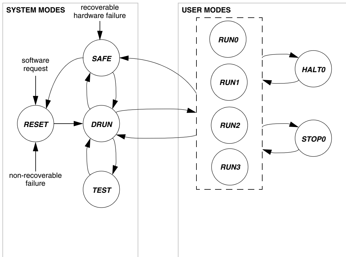
Figure 7-22. MC_ME Mode Diagram
