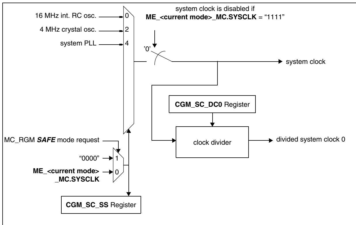
Figure 5-12. MC_CGM System Clock Generation Overview
