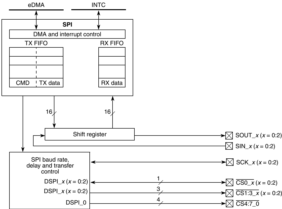
Figure 20-1. DSPI block diagram
