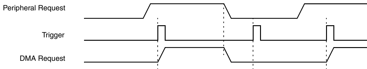
Figure 19-5. DMA mux channel triggering: ignored trigger
