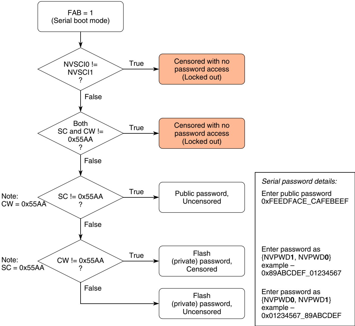
Figure 33-16. Censorship control in serial boot mode
