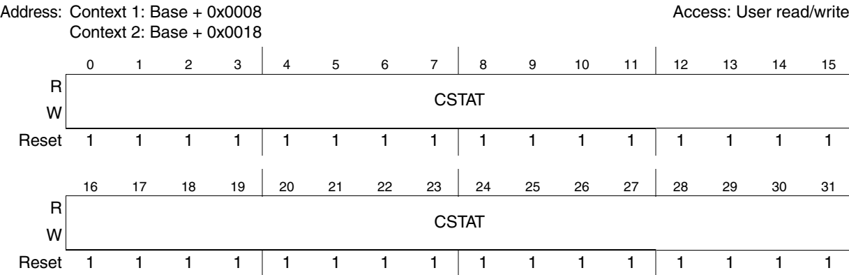
Figure 32-6. CRC Current Status Register (CRC_CSTAT)
