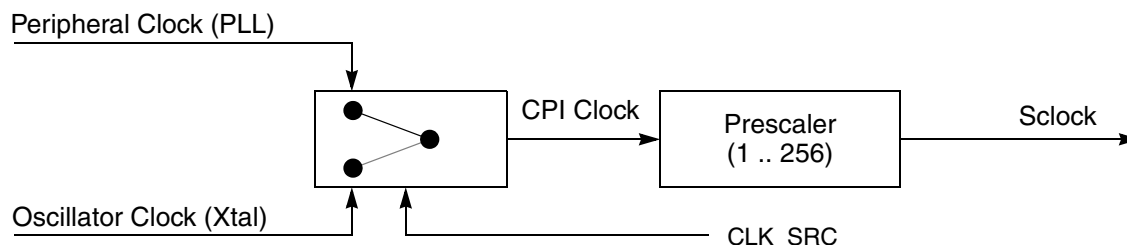
Figure 22-15. CAN engine clocking scheme
