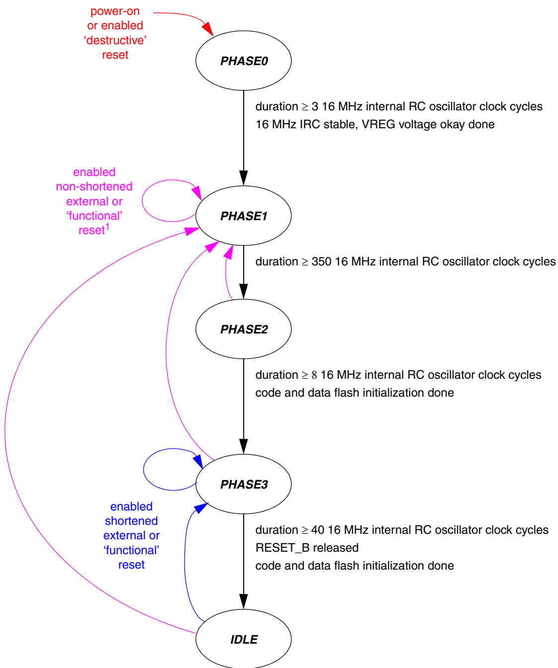
Figure 8-9. MC_RGM State Machine
