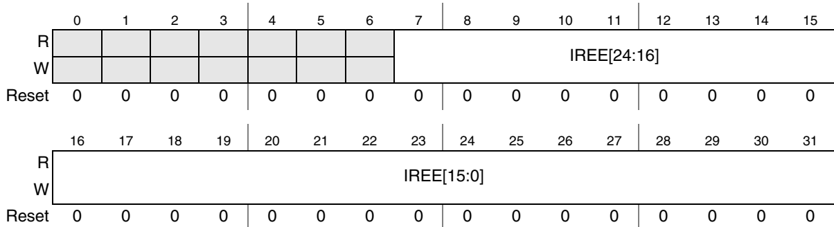
Figure 11-7. Interrupt Rising-Edge Event Enable Register (IREER)
