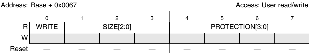
Figure 15-19. RAM ECC Attributes (REAT) register
