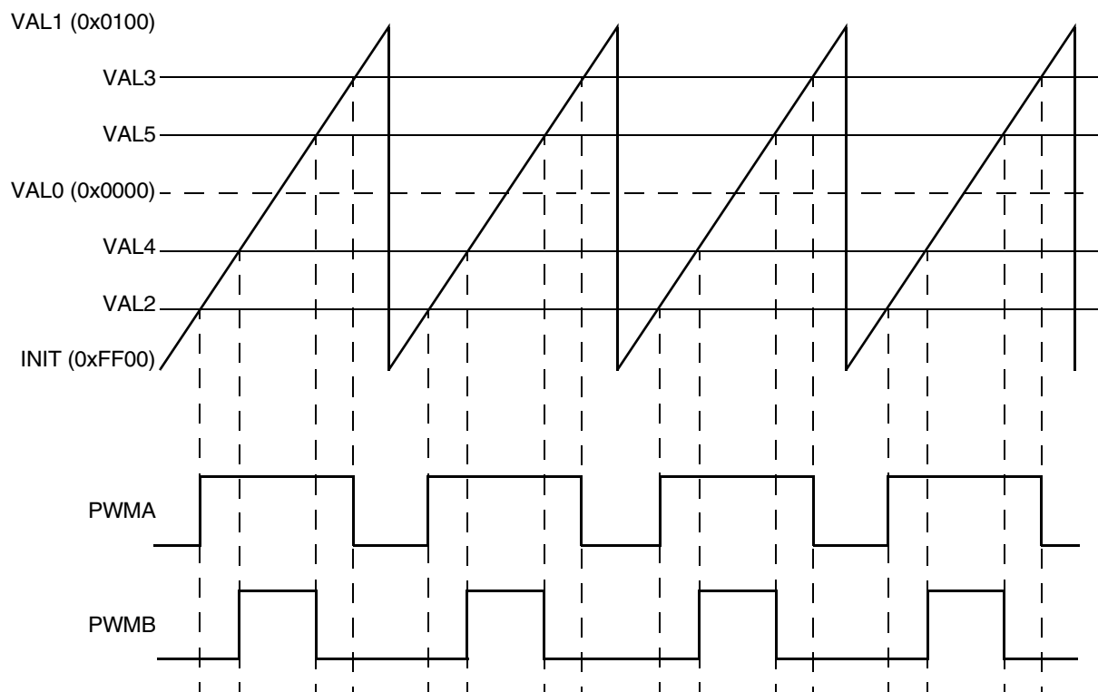
Figure 25-29. Center-aligned example
