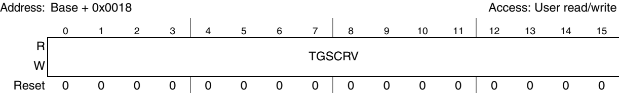
Figure 24-13. TGS Counter Reload Register (TGSCRR)
