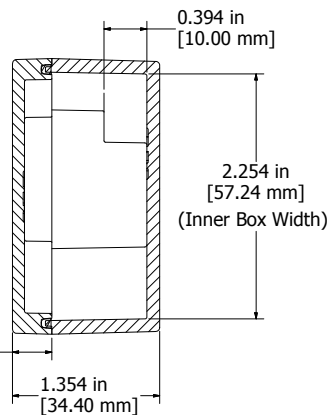
SECTION A-A End View of Assembly
