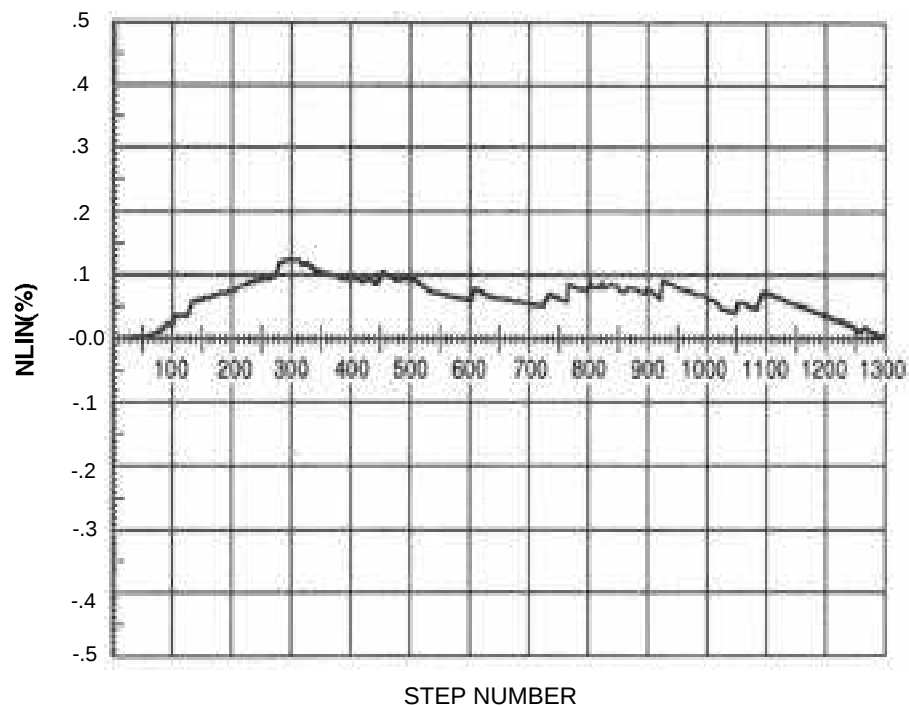
M62362P NONLINEARITY
