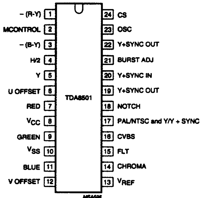
Fig.2 Pin configuration.
