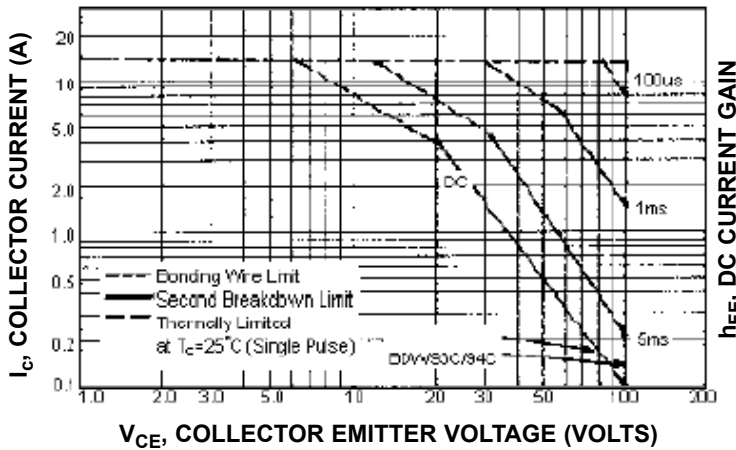
PNP BDW94C
