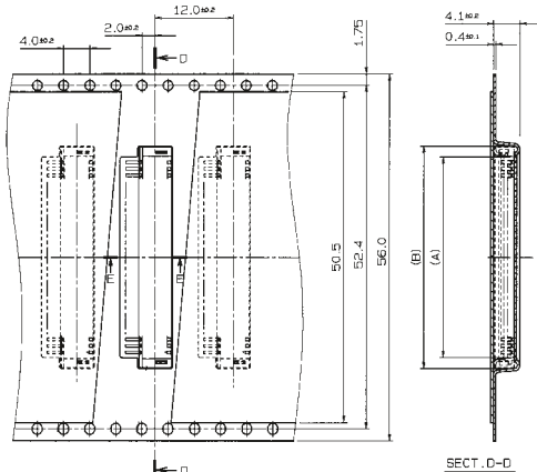
SECT. D-D
