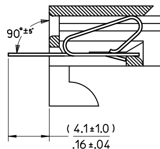
SECTION X-X
