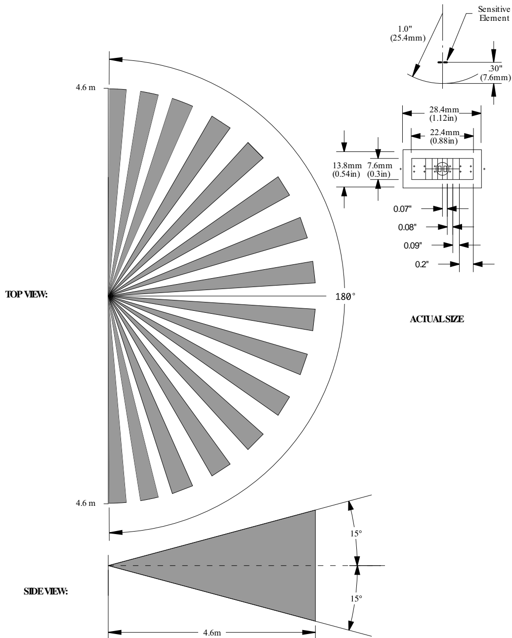
Figure 12. The EWA 0.3 GI V2 Lens Specification, Dimensions
