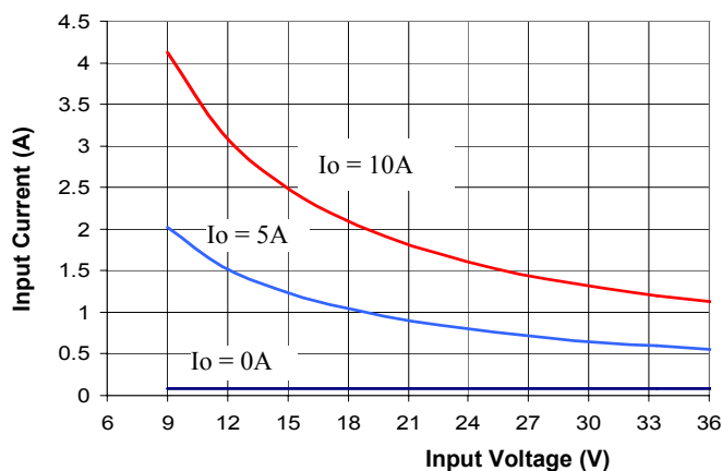
Figure 2. Input Characteristic (3.3V output)
