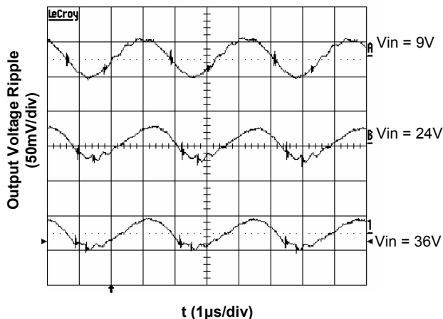
Figure 4. Output Ripple Voltage at 3.3V, 10A Output
