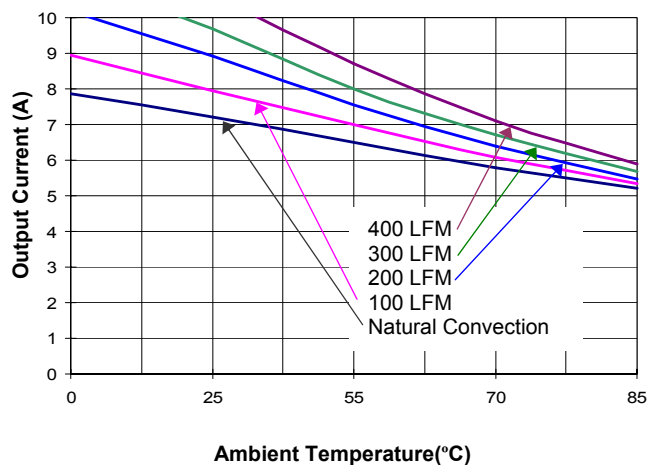
Figure 12(a). Current Derating Curve for 3.3V Output ( V_{in} = 24V open frame)
