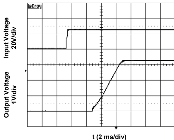
Figure 5. Start-Up from Application of Input Voltage Input voltage 24V, Output current 10A (resistive load) 3.3V
