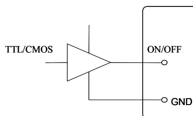
Figure 15. Direct Logic Drive
