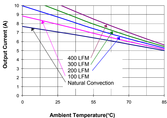
Figure 12(b). Current Derating Curve for 5V Output ( V_{in} = 24V open frame)
