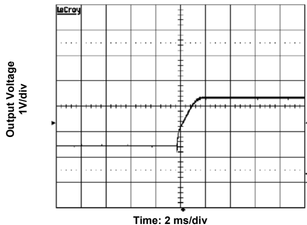
Figure 7. Start-Up with Prebias Input voltage 24V, Output current 0A, Output voltage 3.3V, Prebias 1.5V
