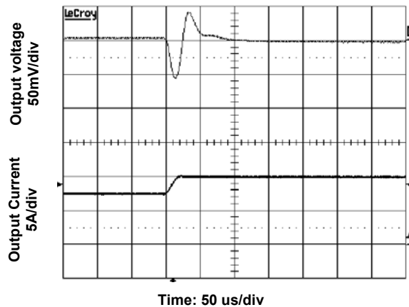
Figure 9. Transient Load Response Input/output voltage 24/3.3V, Output current 7.5A->10A, Slew rate 0.1A/µs .
