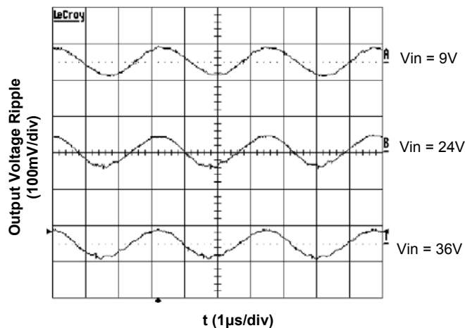
Figure 6. Output Ripple Voltage at 5V, 9A Output
