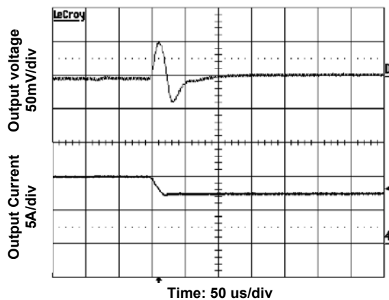
Figure 8. Transient Load Response Input/output voltage 24/3.3V, Output current 10A->7.5A, Slew rate 0.1A/µs.
