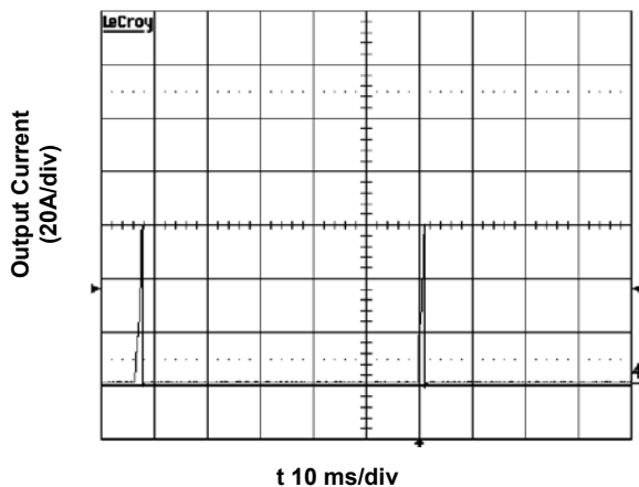
Figure 10. Short Circuit Current. Vin = 24V
