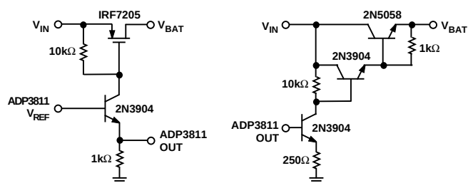
a. P-Channel MOSFET b. NPN Darlington Figure 30. Alternative Pass Transistor for Linear Regulator
