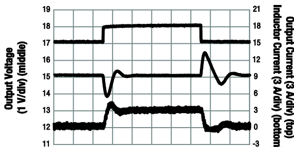
Figure 24. Load Transient ( V_{OUT} = 15 V, V_{IN} = 24 V, I_{OUT} = 0.1 to 3 A)
