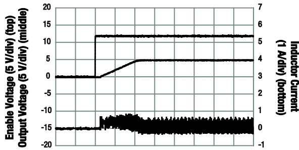
Figure 14. Soft Start ( V_{OUT} = 5\text{ V} , V_{IN} = 12\text{ V} , I_{OUT} = 100\text{ mA} )
