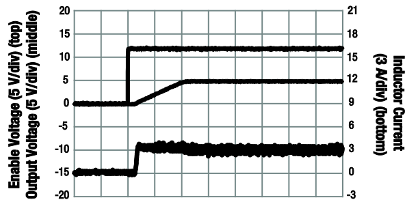
Figure 16. Soft Start ( V_{OUT} = 5\text{ V} , V_{IN} = 12\text{ V} , I_{OUT} = 3\text{ A} )
