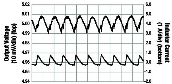
Figure 19. Output Voltage Ripple ( V_{OUT} = 5\text{ V} , V_{IN} = 24\text{ V} , I_{OUT} = 100\text{ mA} )
