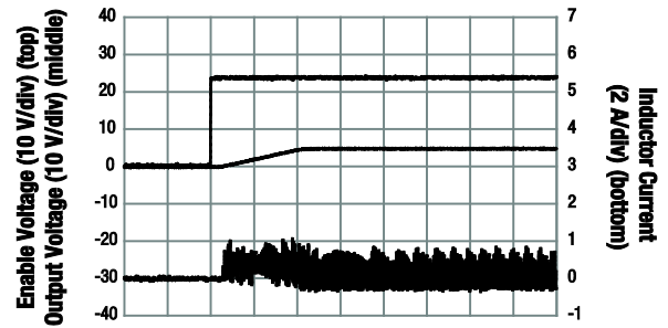
Figure 15. Soft Start ( V_{OUT} = 5\text{ V} , V_{IN} = 24\text{ V} , I_{OUT} = 100\text{ mA} )
