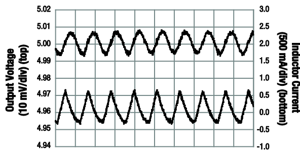
Figure 18. Output Voltage Ripple ( V_{OUT} = 5\text{ V} , V_{IN} = 12\text{ V} , I_{OUT} = 100\text{ mA} )
