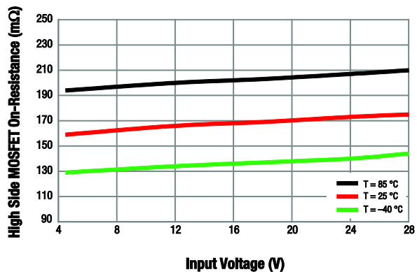
Figure 13. High Side MOSFET On-Resistance vs Input Voltage
