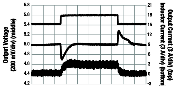
Figure 23. Load Transient ( V_{OUT} = 5 V, V_{IN} = 24 V, I_{OUT} = 0.1 to 3 A)
