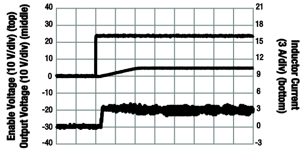
Figure 17. Soft Start ( V_{OUT} = 5\text{ V} , V_{IN} = 24\text{ V} , I_{OUT} = 3\text{ A} )
