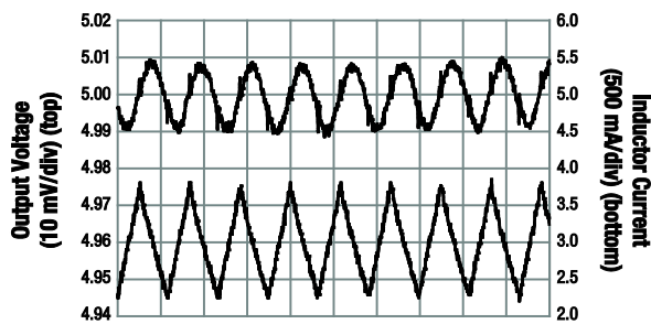
Figure 20. Output Voltage Ripple ( V_{OUT} = 5 V, V_{IN} = 12 V, I_{OUT} = 3 A)
