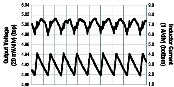
Figure 21. Output Voltage Ripple ( V_{OUT} = 5 V, V_{IN} = 24 V, I_{OUT} = 3 A)
