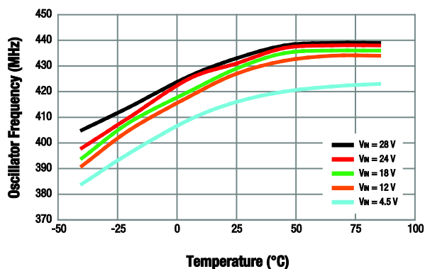
Figure 10. Oscillator Frequency vs Temperature ( I_{out} = 100\text{ mA} )
