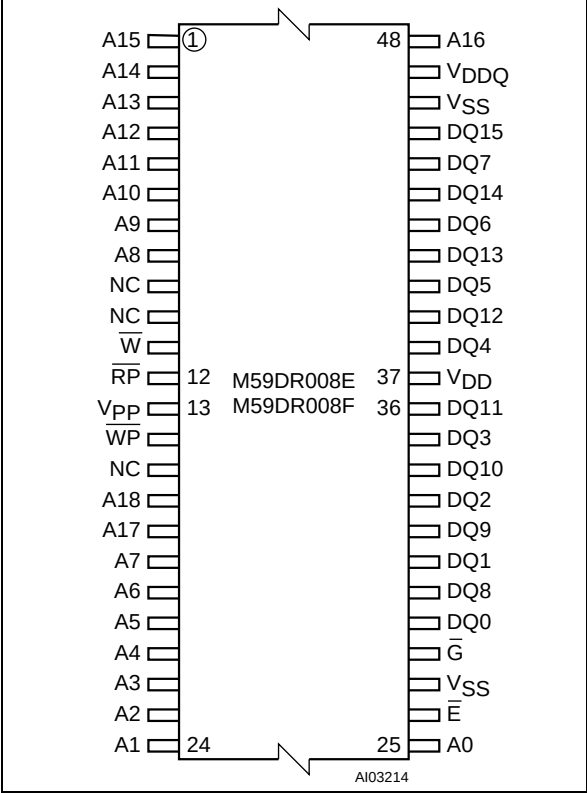
Figure 3. TSOP Connections
