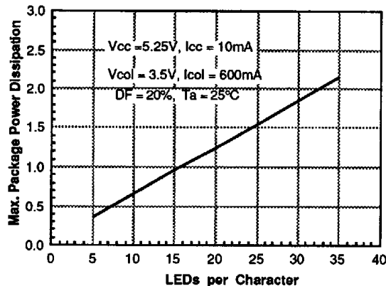
FIGURE 8. MAX. PACKAGE POWER DISSIPATION
