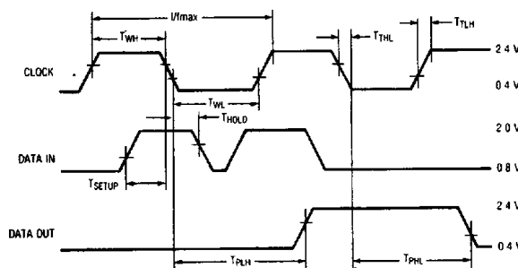
FIGURE 1. TIMING CHARACTERISTICS
