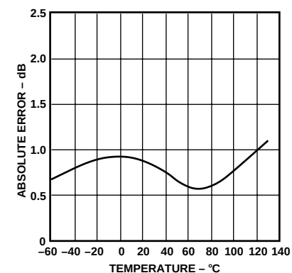
Figure 9. Absolute Error vs. Temperature, Using Attenuator. V_{IN} = \pm 10 mV to \pm 1 V, Pin 8 Grounded to Disable ITC Bias
