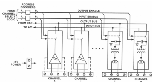
Figure 1 5B08 MUX Functional Block Diagram
