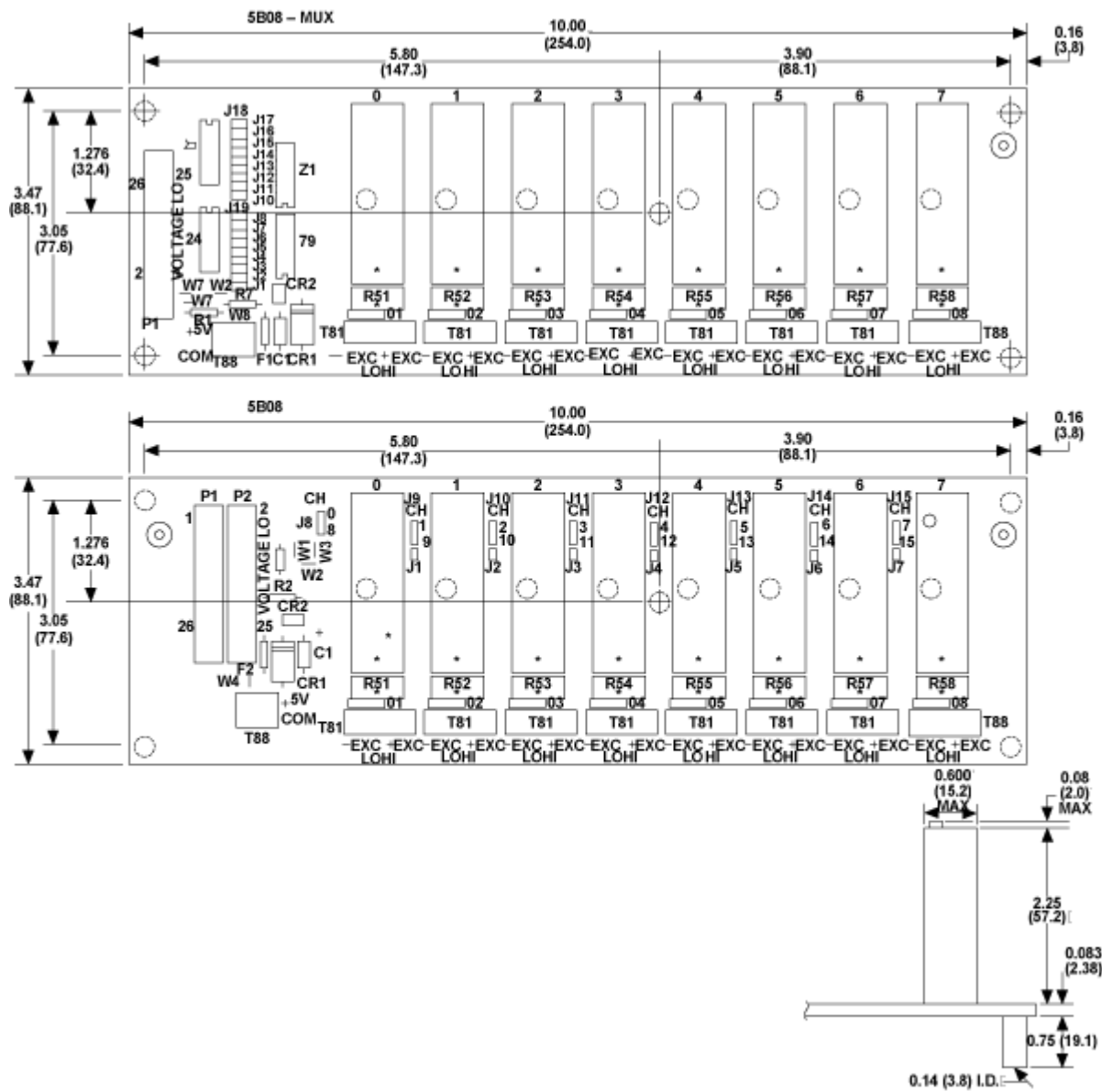
Figure 5 Outline Dimensions
