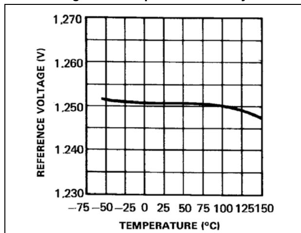
Figure 7. Temperature stability
