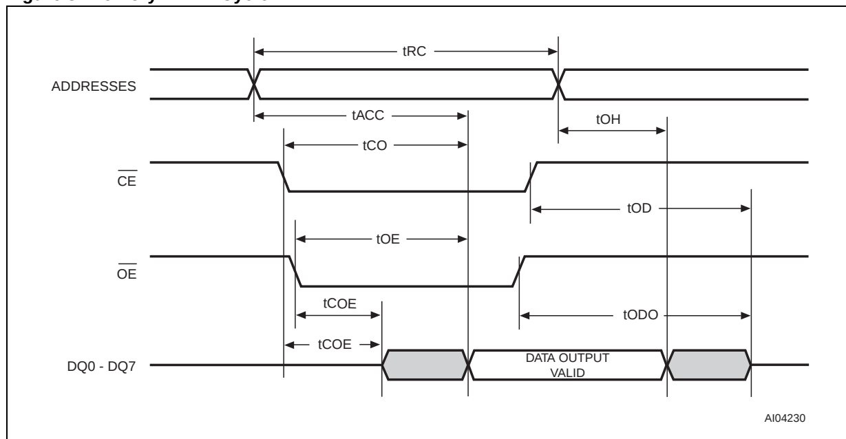
Figure 8. Memory READ Cycle
