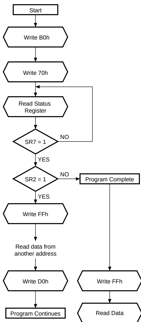
Figure 24. Program Suspend &amp; Resume Flowchart and Pseudo Code
