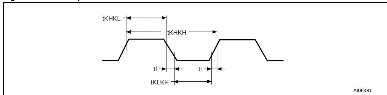
Figure 14. Clock input AC Waveform
