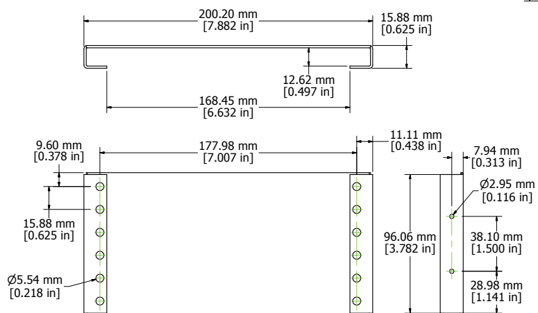
END PLATES
