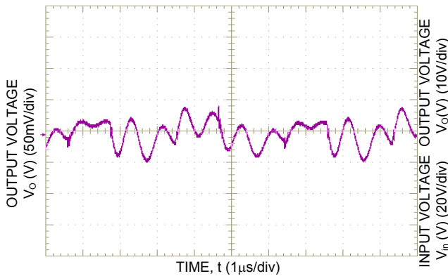
Figure 2. Typical Output Ripple and Noise at Room Temperature and 48Vin; I_o = I_{o,max} ; C_{o,ext} = 440\mu F .
