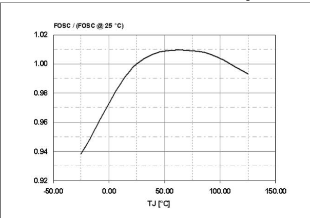
Figure 7. Switching frequency vs T_J
