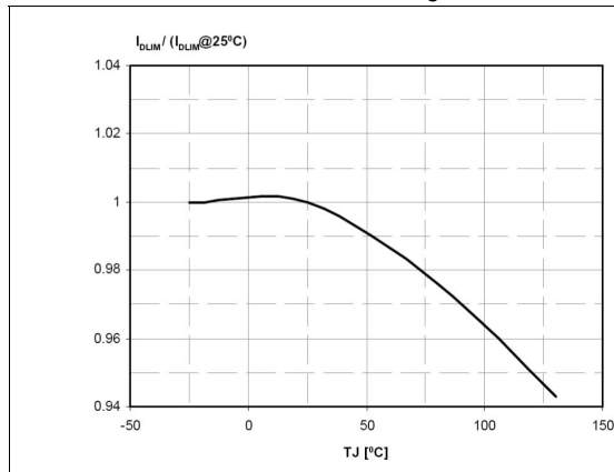
Figure 6. Current limit vs T_J
