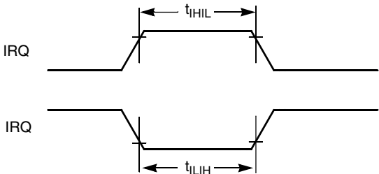
Figure 5. IRQ Timing
