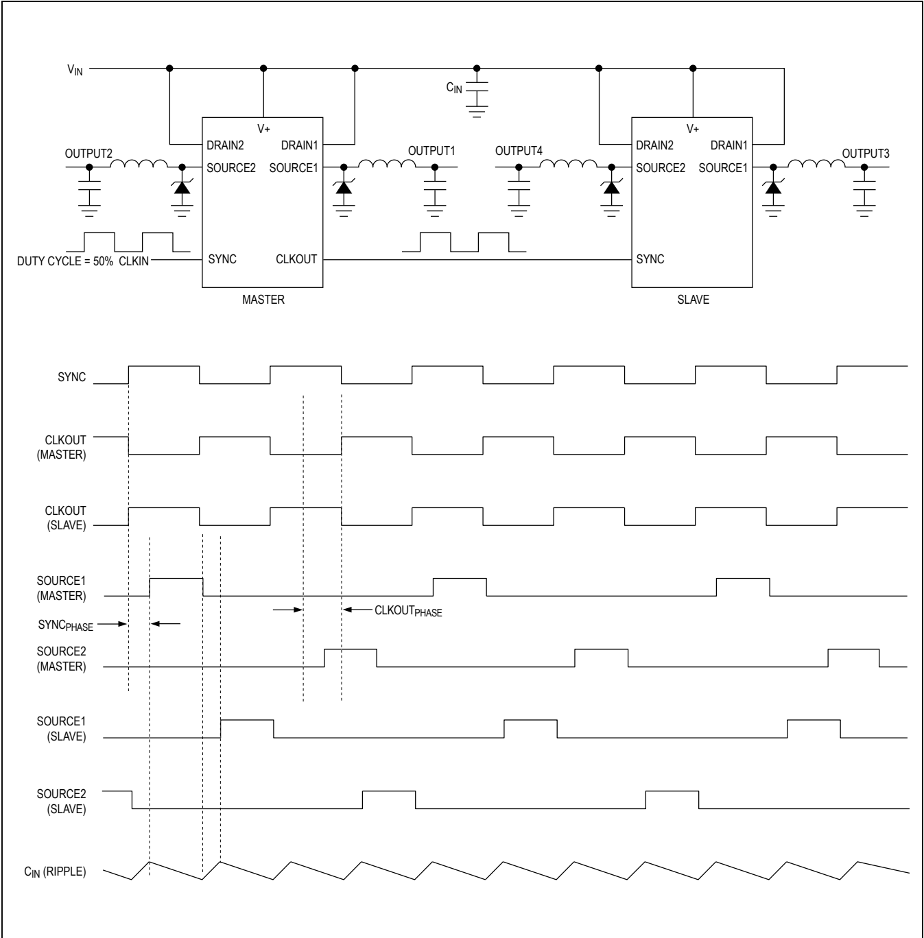
Figure 3. Synchronized Controllers
