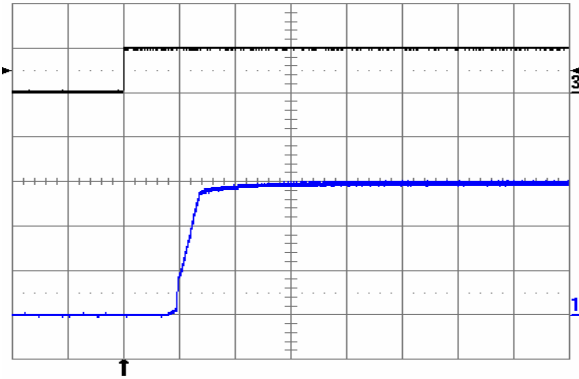
Fig. 5: Turn-on transient at full rated load current (resistive) with no output capacitor at V_{in} = 48\text{ V} , triggered via ON/OFF pin. Top trace: ON/OFF signal (5 V/div.). Bottom trace: output voltage (0.5 V/div.) Time scale: 2 ms/div.
