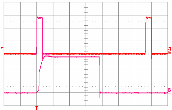
Fig. 13: Load current (top trace, 20 A/div, 20 ms/div) into a 10 m \Omega short circuit during restart, at V_{in} = 48 V. Bottom trace (20 A/div, 1 ms/div) is an expansion of the on-time portion of the top trace.
