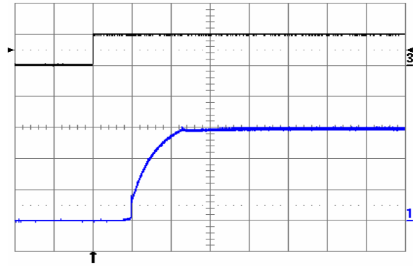
Fig. 6: Turn-on transient at full rated load current (resistive) plus 40,000 \mu\text{F} at V_{in} = 48\text{ V} , triggered via ON/OFF pin. Top trace: ON/OFF signal (5 V/div.). Bottom trace: output voltage (0.5 V/div.) Time scale: 2 ms/div.
