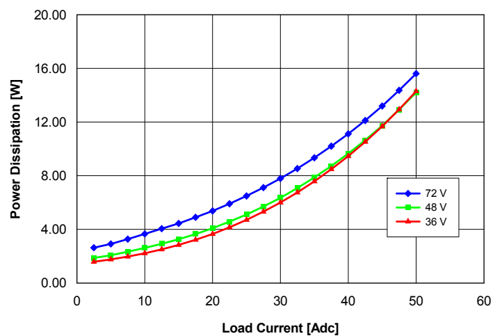
Fig. 4: Power dissipation vs. load current and input voltage for converter mounted vertically with air flowing from pin 3 to pin 1 at a rate of 300 LFM (1.5 m/s) and T_a = 25^{\circ}\text{C} .
