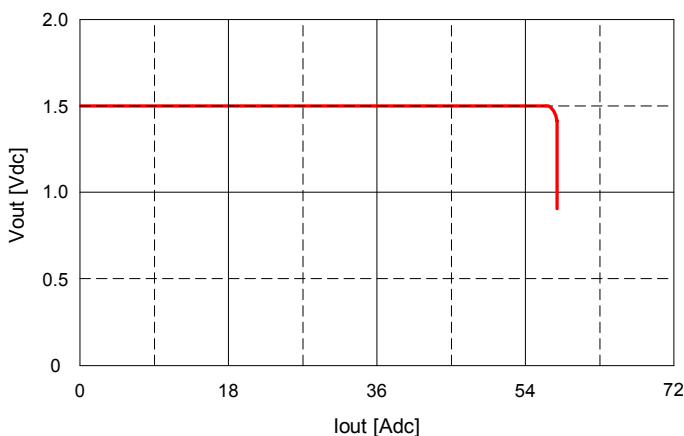
Fig. 12: Output voltage vs. load current showing current limit point and converter shutdown point. Input voltage has almost no effect on current limit characteristic.
