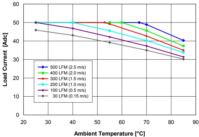
Fig. 1: Available load current vs. ambient air temperature and airflow rates for QM48T50015 converter with D height pins mounted vertically with air flowing from pin 3 to pin 1, MOSFET temperature \leq 120^{\circ}\text{C} , V_{in} = 48\text{ V} .
