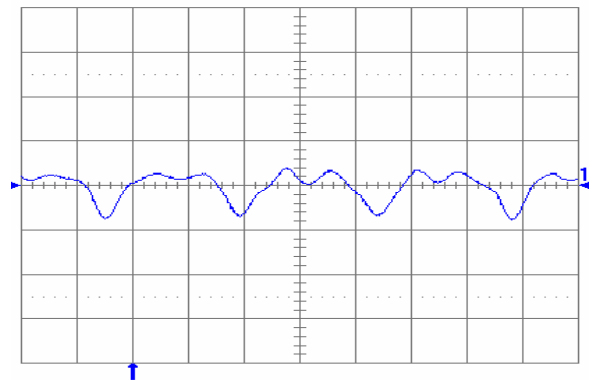
Fig. 8: Output voltage ripple (20 mV/div.) at full rated load current into a resistive load with C_o = 10\text{ }\mu\text{F} tantalum + 1 \mu\text{F} ceramic and V_{in} = 48\text{ V} . Time scale: 1 \mu\text{s} /div.
