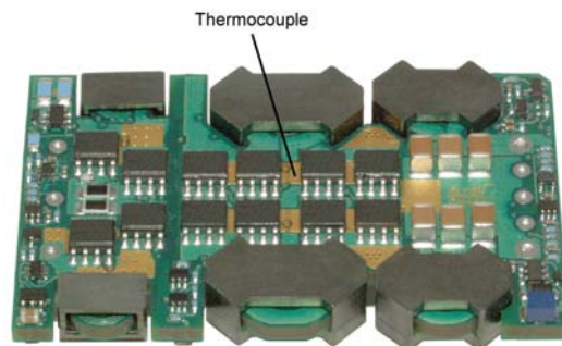
Fig. H: Location of the thermocouple for thermal testing.
