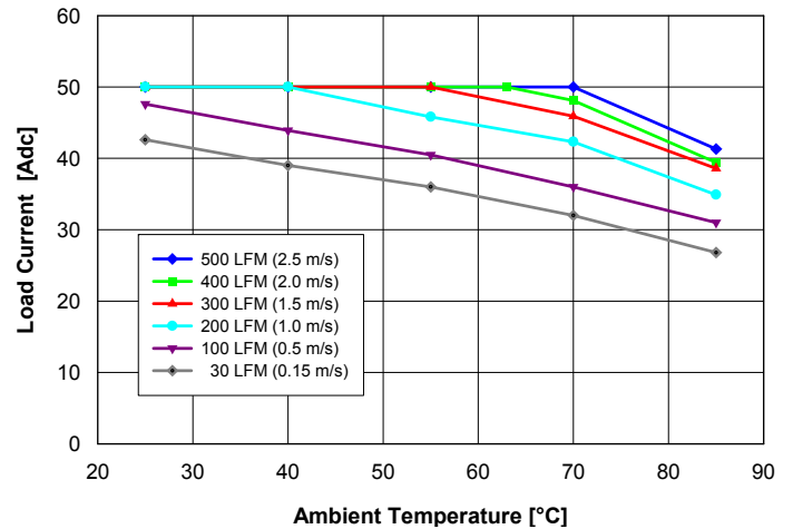
Fig. 2: Available load current vs. ambient air temperature and airflow rates for QM48T50015 converter with D height pins mounted horizontally with air flowing from pin 3 to pin 1, MOSFET temperature \leq 120^{\circ}\text{C} , V_{in} = 48\text{ V} .
