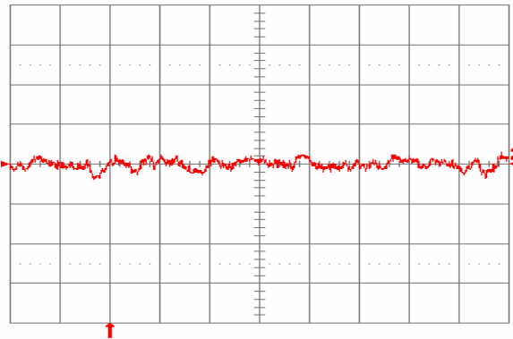
Fig. 10: Input reflected ripple current, i_s (10 mA/div), measured through 10 \mu H at the source at full rated load current and V_{in} = 48 V. Refer to Fig. 9 for test setup. Time scale: 1 \mu s/div.
