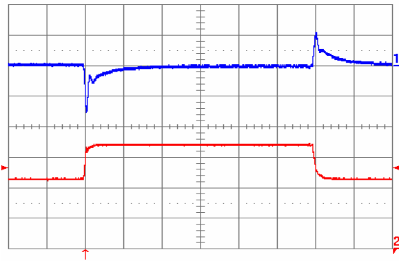
Fig. 7: Output voltage response to load current step-change (25 A – 37.5 A – 25 A) at V_{in} = 48\text{ V} . Top trace: output voltage (100 mV/div.). Bottom trace: load current (10 A/div.). Current slew rate: 1 A/ \mu\text{s} . C_o = 470\text{ }\mu\text{F} tantalum + 1 \mu\text{F} ceramic. Time scale: 0.2 ms/div.
