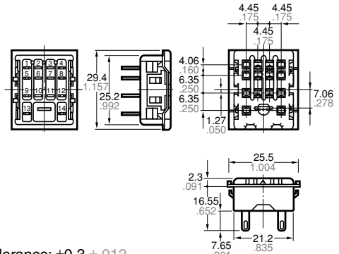
External dimensions
