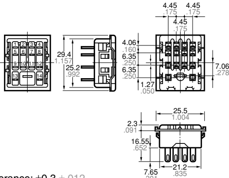
External dimensions
