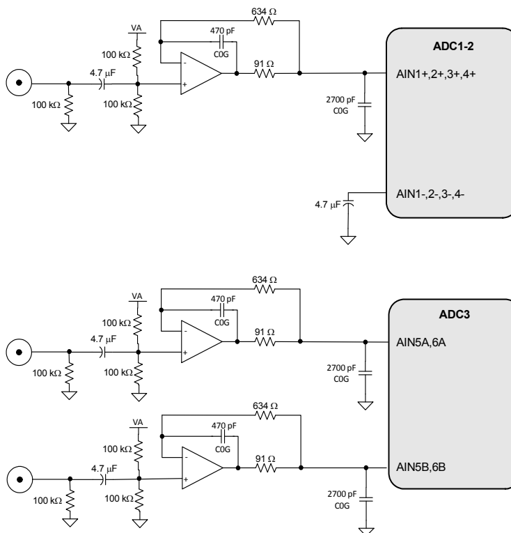
Figure 27. Single-Ended Active Input Filter
