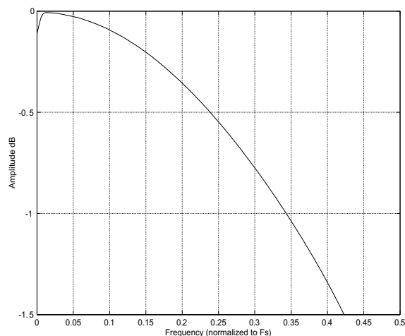
Figure 55. QSM Passband Ripple
