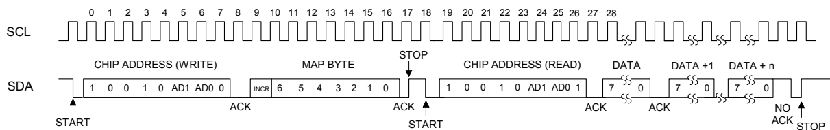
Figure 25. Control Port Timing, I²C Read
