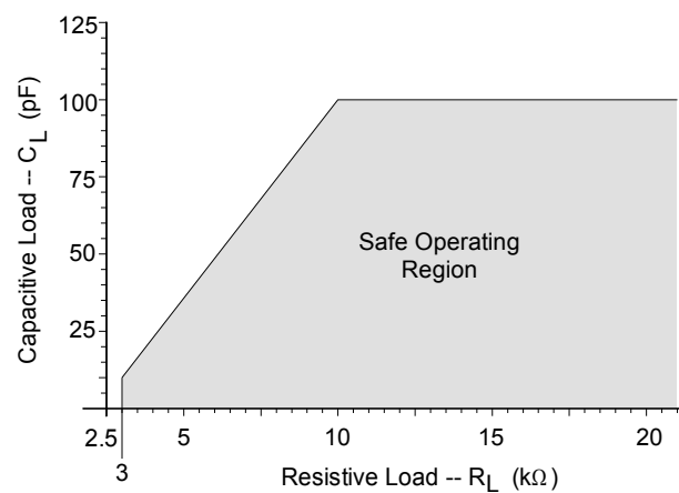
Figure 3. Maximum Loading
