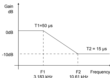
Figure 14. De-Emphasis Curve
