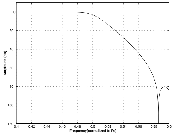
Figure 48. Double-Speed (fast) Transition Band
