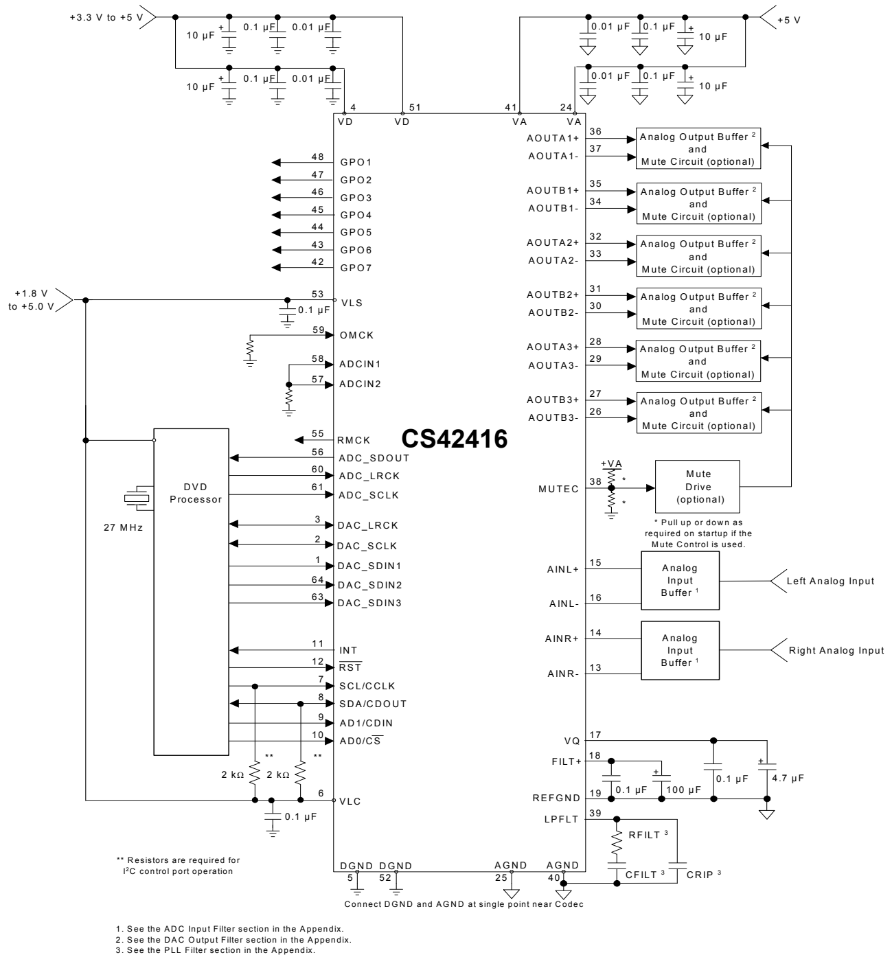
Figure 6. Typical Connection Diagram using the PLL
