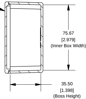
SECTION A-A End View of Assembly
