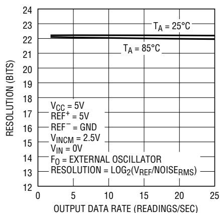
Figure 31. Resolution (Noise RMS ≤ 1LSB) vs Output Data Rate and Temperature
