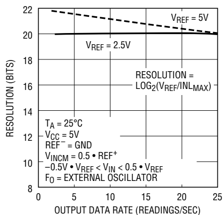
Figure 35. Resolution (INL MAX ≤ 1LSB) vs Output Data Rate and Reference Voltage
