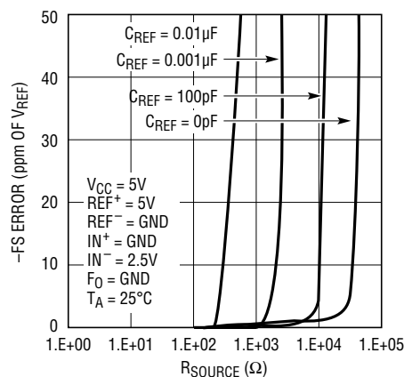
Figure 24. -FS Error vs R SOURCE at REF + or REF - (Small C REF )
