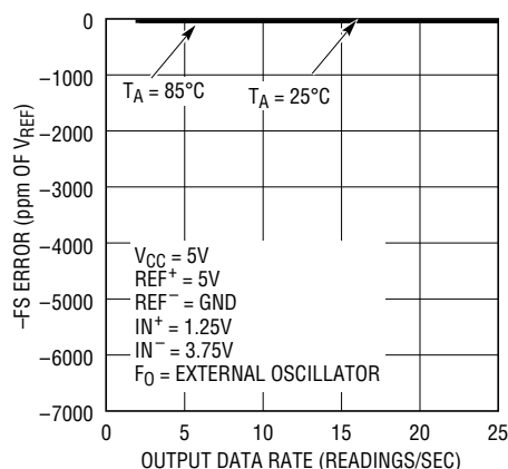
Figure 30. -FS Error vs Output Data Rate and Temperature
