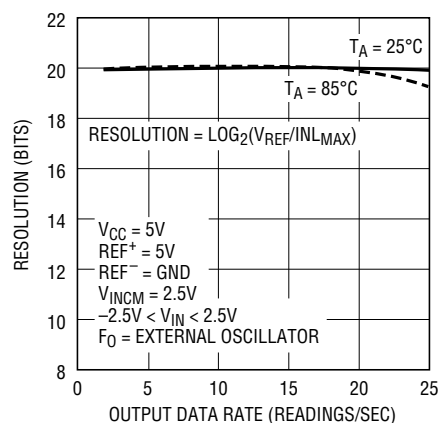
Figure 32. Resolution (INL RMS ≤ 1LSB) vs Output Data Rate and Temperature
