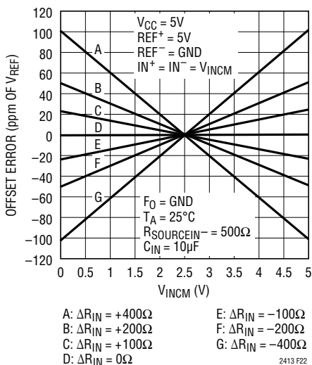
Figure 22. Offset Error vs Common Mode Voltage ( V_{INCM} = IN^+ = IN^- ) and Input Source Resistance Imbalance ( \Delta R_{IN} = R_{SOURCEIN+} - R_{SOURCEIN-} ) for Large C_{IN} Values ( C_{IN} \geq 1\mu F )
