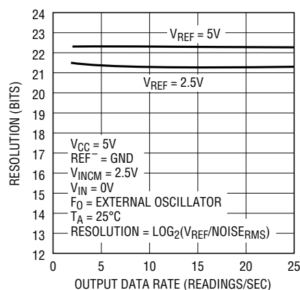
Figure 34. Resolution (Noise RMS ≤ 1LSB) vs Output Data Rate and Reference Voltage
