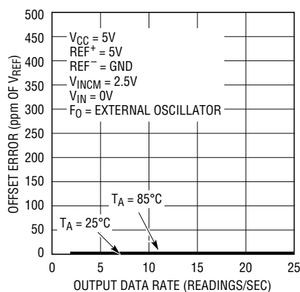
Figure 28. Offset Error vs Output Data Rate and Temperature
