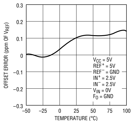
Offset Error vs Temperature ( T_A )
