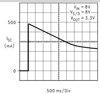
Figure 9. Turnon Waveform
