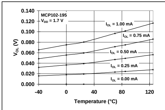
FIGURE 2-19: V_{OL} vs. Temperature (MCP102-195 @ V_{DD} = 1.7\text{V} ).
