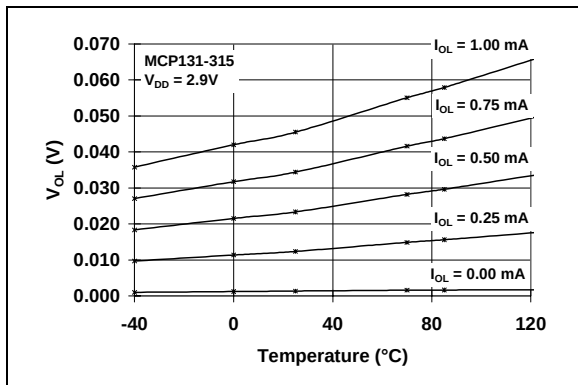
FIGURE 2-20: V_{OL} vs. Temperature (MCP131-315 @ V_{DD} = 2.9\text{V} ).
