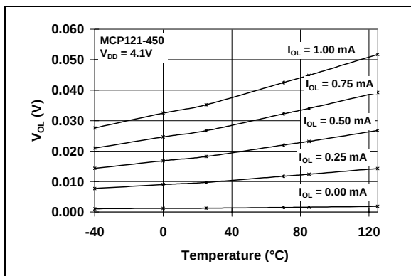
FIGURE 2-21: V_{OL} vs. Temperature (MCP121-450 @ V_{DD} = 4.1\text{V} ).
