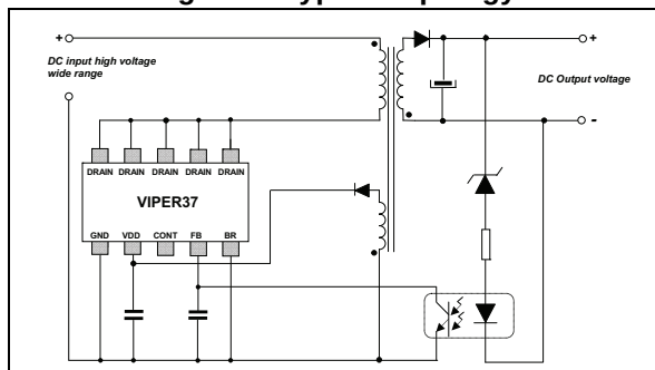
Figure 1. Typical topology
