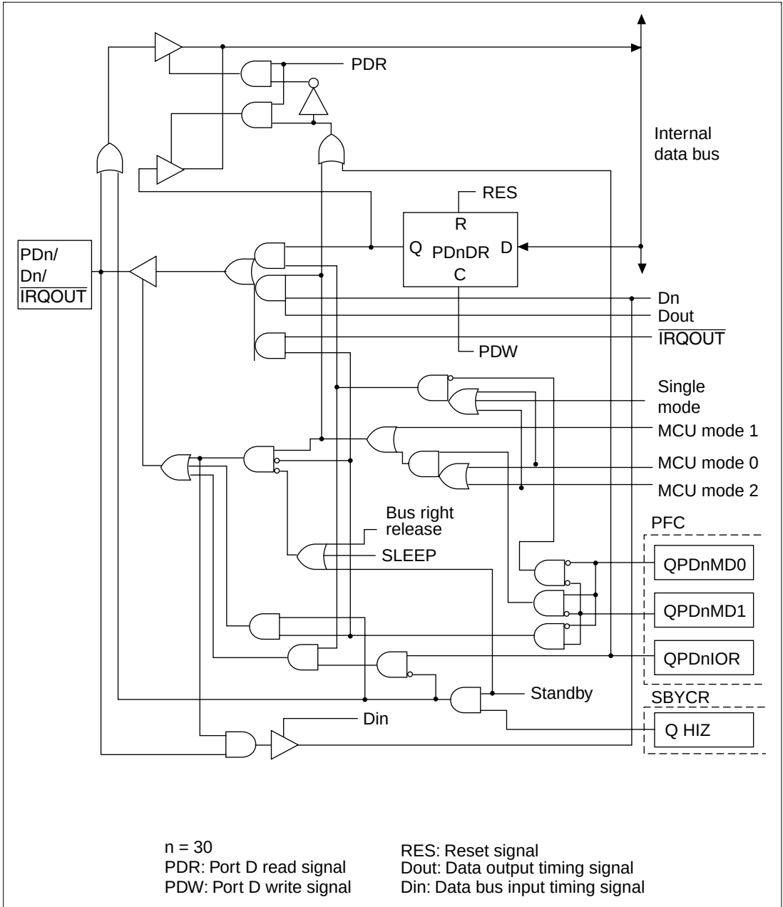
Figure B.30 PDn/Dn/IRQOUT Block Diagram (n = 30)
