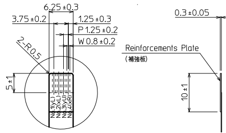
DETAIL B (2:1)
