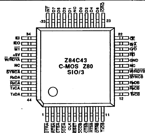
Figure 7b. 44-Pin LOFP Pin Assignments
