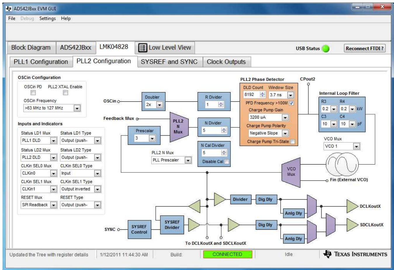
Figure 9. LMK04828 PLL2 Controls
