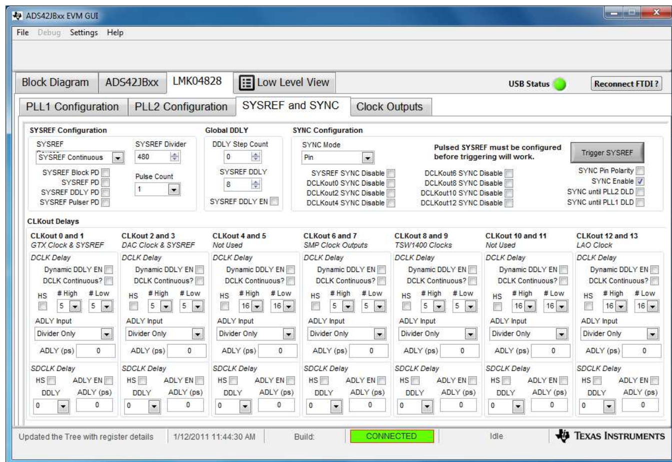
Figure 10. LMK04828 SYSREF and SYNC Settings
