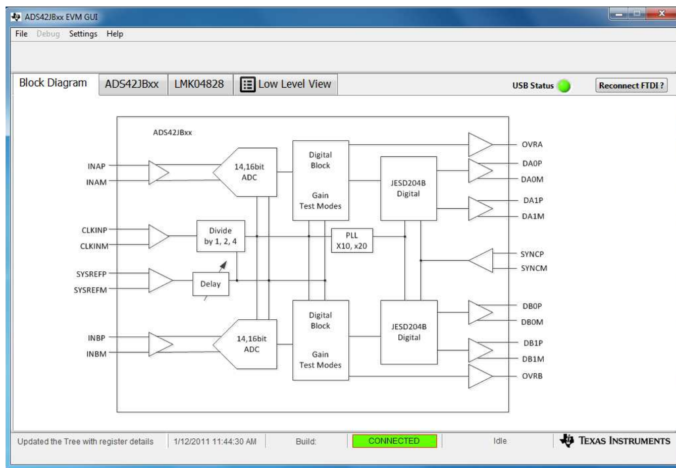
Figure 6. Top-Level Block Diagram Window of the ADS42JBxx GUI
