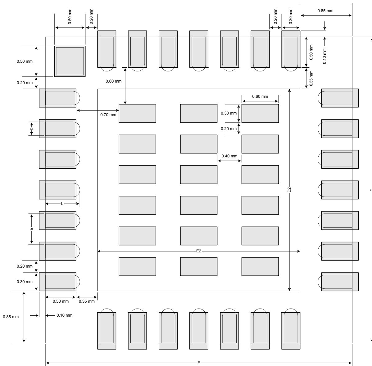
Figure 4.4. Typical MLP-28 Solder Mask
