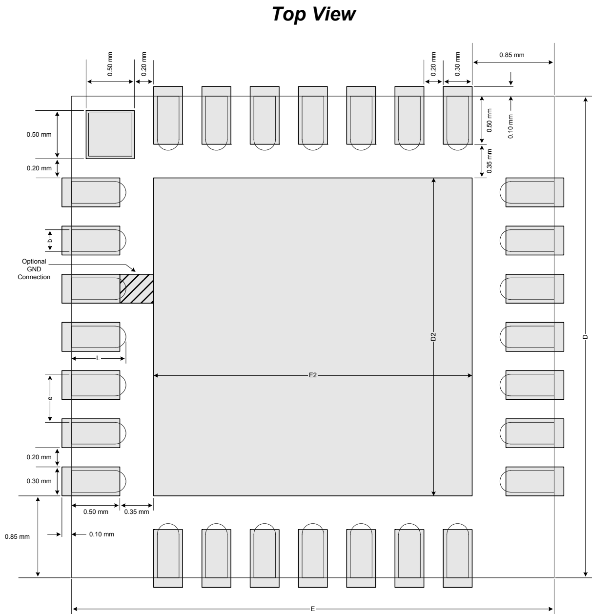
Figure 4.3. Typical MLP-28 Landing Diagram
