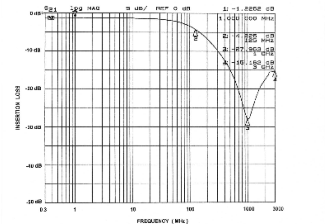
Figure 3. Insertion Loss vs. Frequency Performance Curve, PACUSBVBD2 (SOT23-
