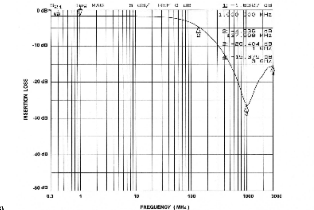
Figure 4. Insertion Loss vs. Frequency Performance Curve, PACUSBVBD3 (SOT23-6)
