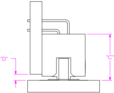
FIG 3 SFM-D-SM MATED WITH TFM-D-RA NOTES:
