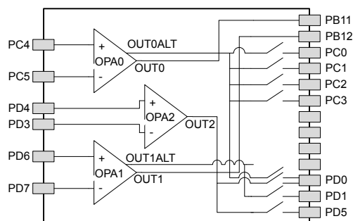
Figure 5.40. Opamp Pinout
