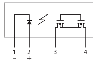
CPC1926Y Pinout
