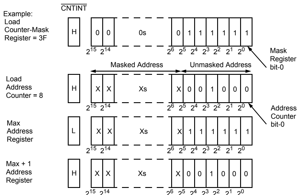
Figure 2. Programmable Counter-Mask Register Operation [17]
