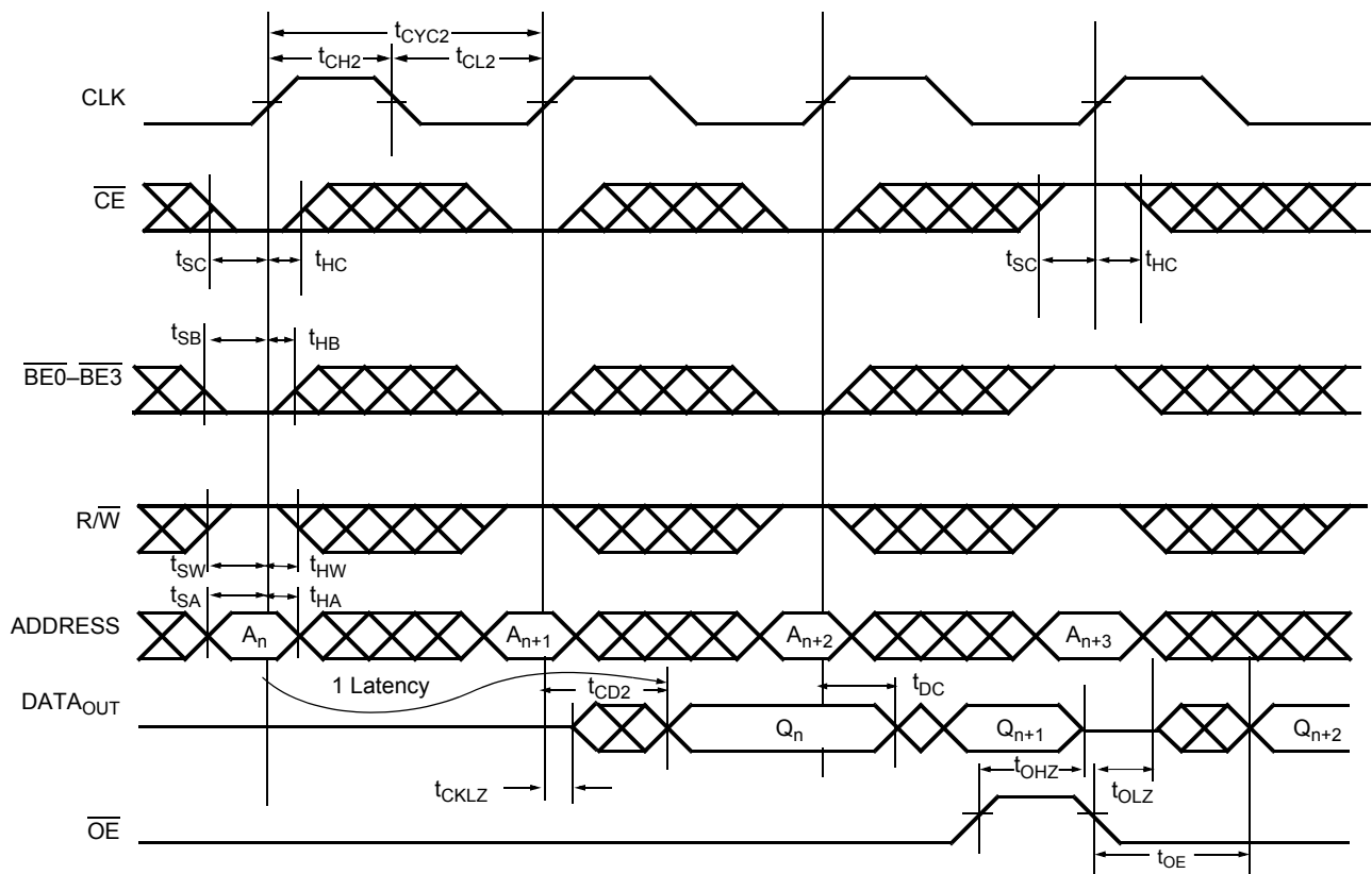
Figure 7. Read Cycle [27, 28, 29, 30, 31]
