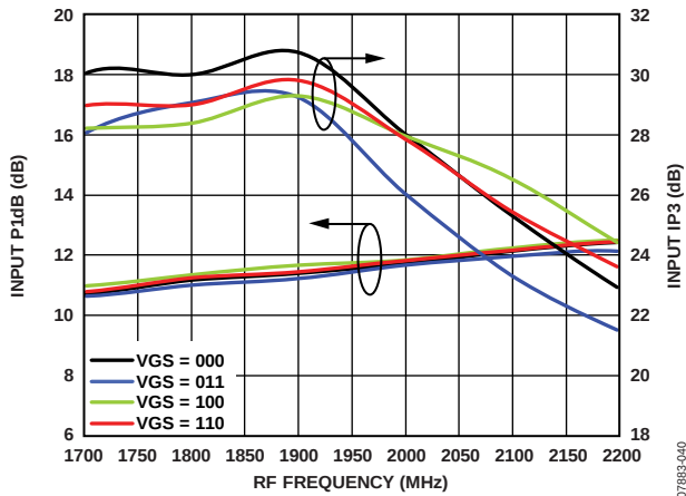
Figure 40. Input IP3 and Input P1dB vs. RF Frequency for Various VGS Settings
