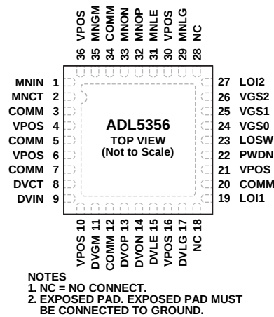
Figure 2. Pin Configuration
