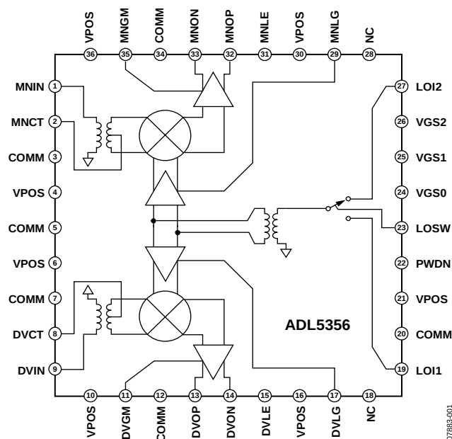
Figure 52. Simplified Schematic
