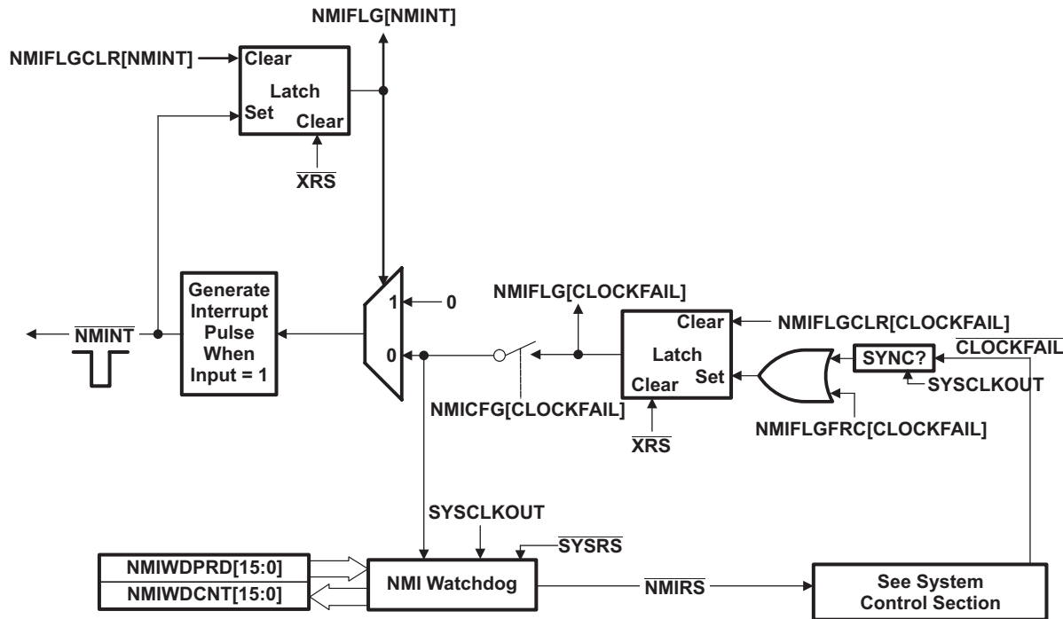
Figure 6-10. NMI Watchdog
