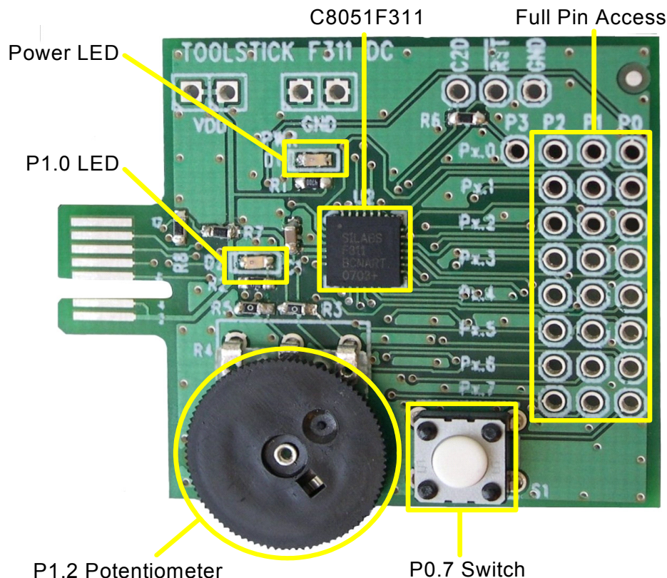
Figure 3. ToolStick C8051F311 Daughter Card
