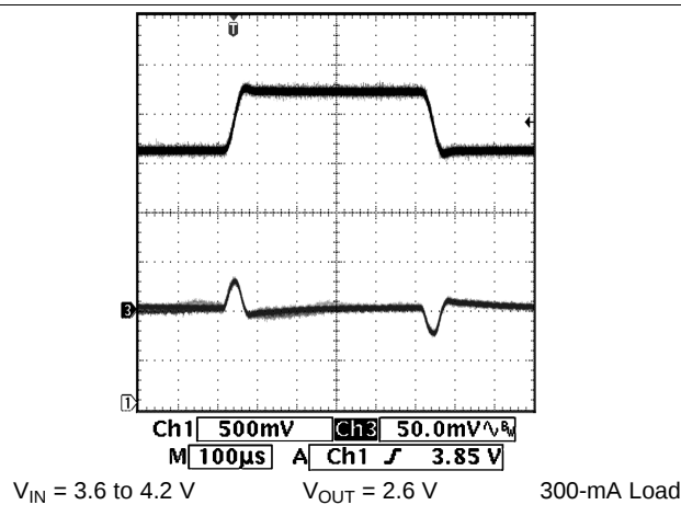
Figure 5. Line Transient (LDO1)
