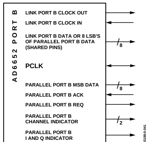
Figure 54. Output Port Configuration
