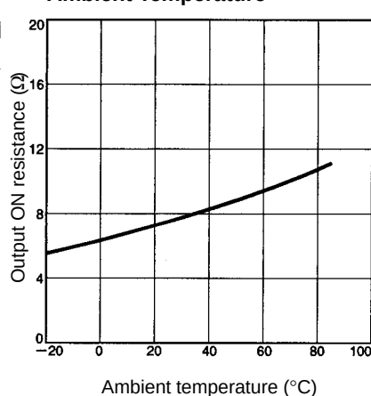
Output ON Resistance vs. Ambient Temperature
