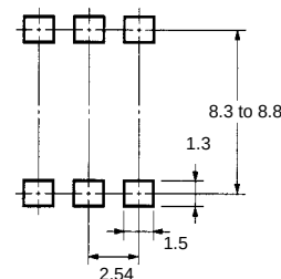
Actual Mounting Pad Dimensions (Recommended Value, Top View)
