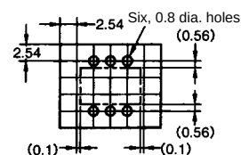
Actual Mounting Pad Dimensions (Recommended Value, Top View)
