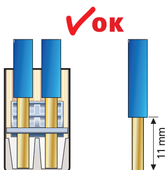
Solid 1.0 - 2.5 mm 2
